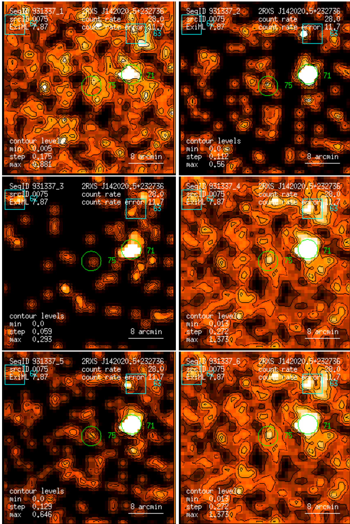
Figure 75: RASS 931337: detection 0075: band rate images, Gaussian filter: (1) PSPC channels 11 – 41, (2) 52 – 90, (3) 91 – 201, (4) 11 – 235, (5) 52 – 201, (6) 11 – 201. Broad band rates in counts/ks. Band rate contour levels in counts/ks/arcmin 2 .
