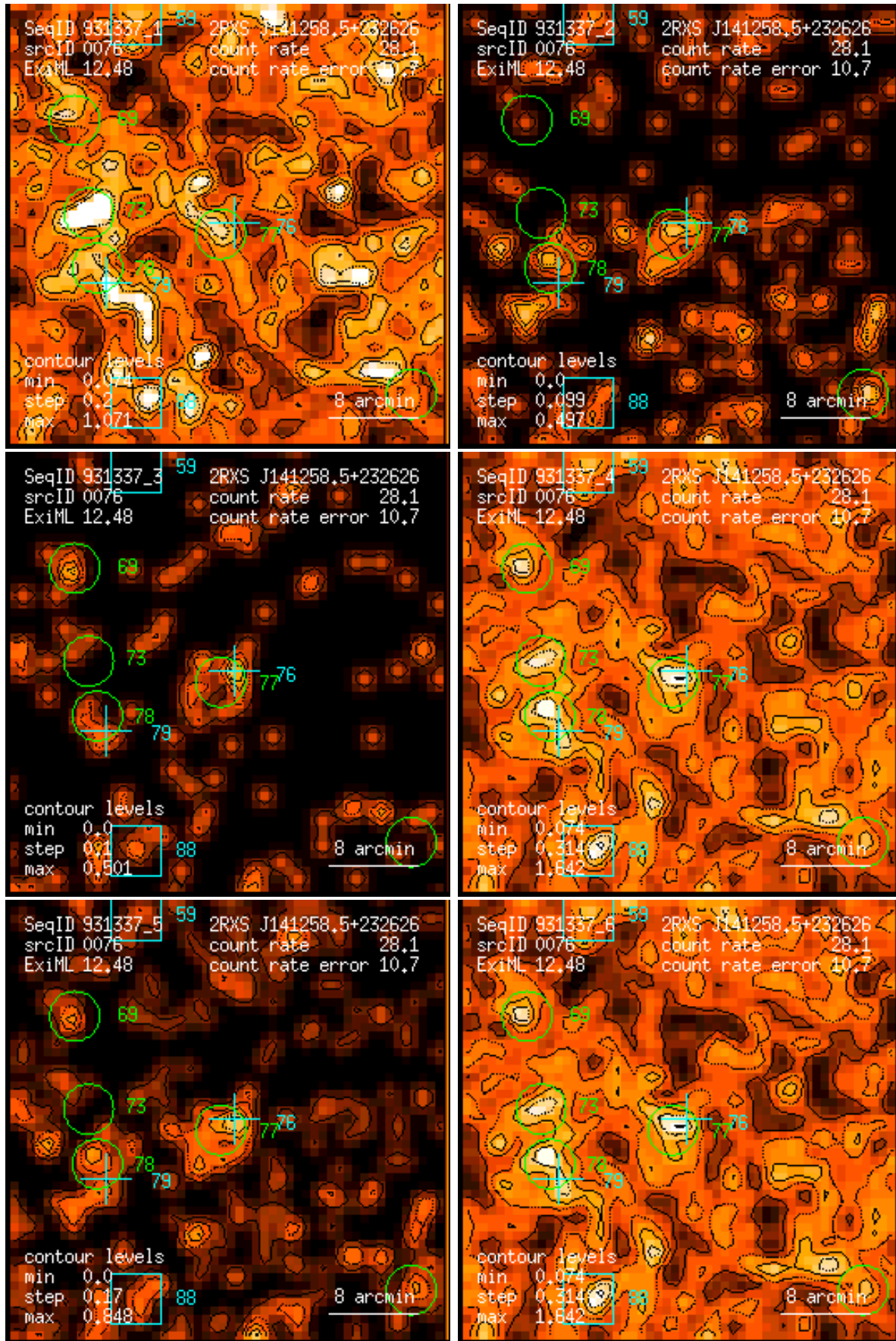
Figure 76: RASS 931337: detection 0076: band rate images, Gaussian filter: (1) PSPC channels 11 – 41, (2) 52 – 90, (3) 91 – 201, (4) 11 – 235, (5) 52 – 201, (6) 11 – 201. Broad band rates in counts/ks. Band rate contour levels in counts/ks/arcmin 2 .
