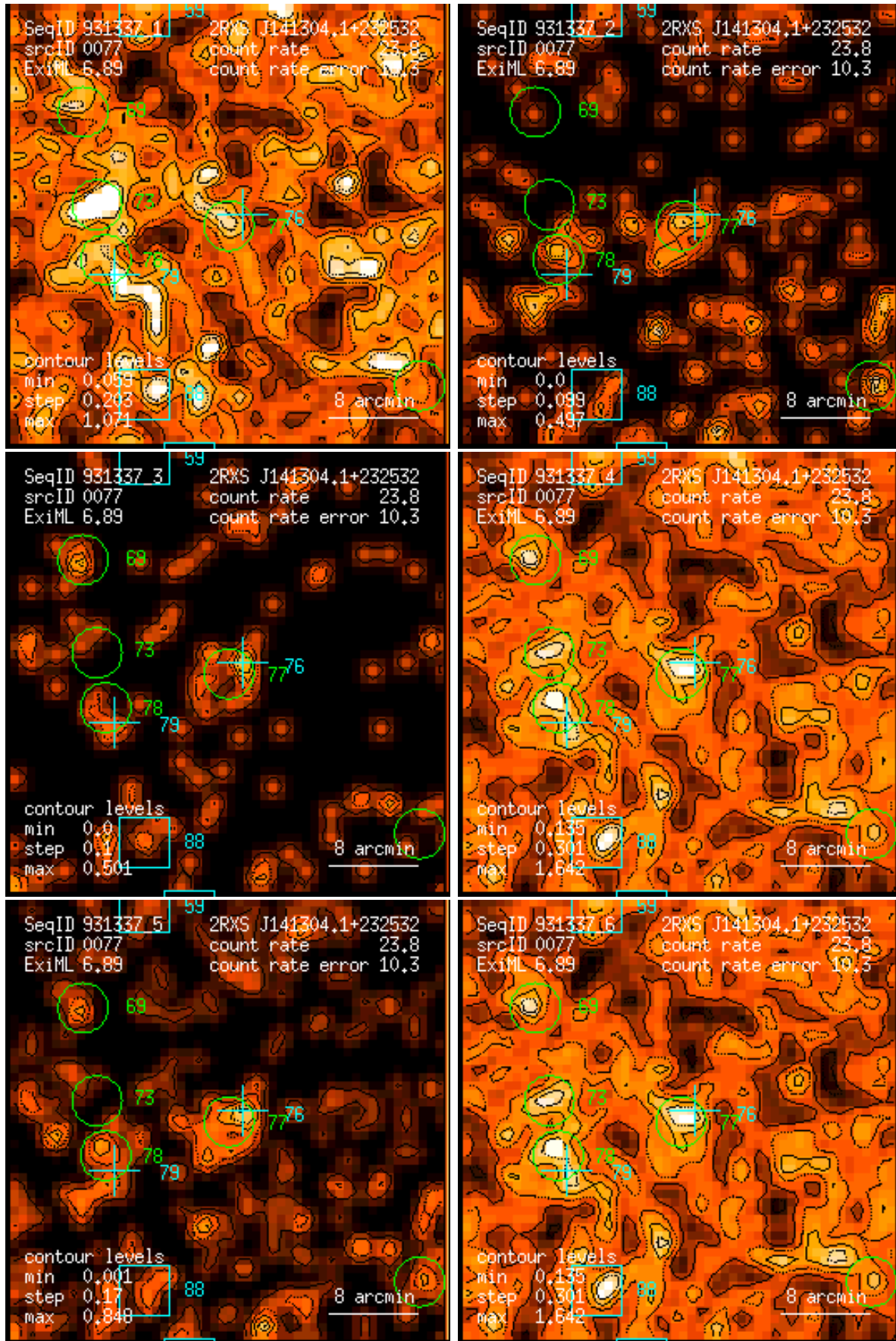
Figure 77: RASS 931337: detection 0077: band rate images, Gaussian filter: (1) PSPC channels 11 – 41, (2) 52 – 90, (3) 91 – 201, (4) 11 – 235, (5) 52 – 201, (6) 11 – 201. Broad band rates in counts/ks. Band rate contour levels in counts/ks/arcmin 2 .
