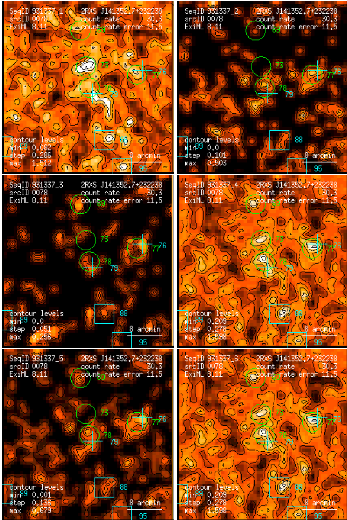
Figure 78: RASS 931337: detection 0078: band rate images, Gaussian filter: (1) PSPC channels 11 – 41, (2) 52 – 90, (3) 91 – 201, (4) 11 – 235, (5) 52 – 201, (6) 11 – 201. Broad band rates in counts/ks. Band rate contour levels in counts/ks/arcmin 2 .
