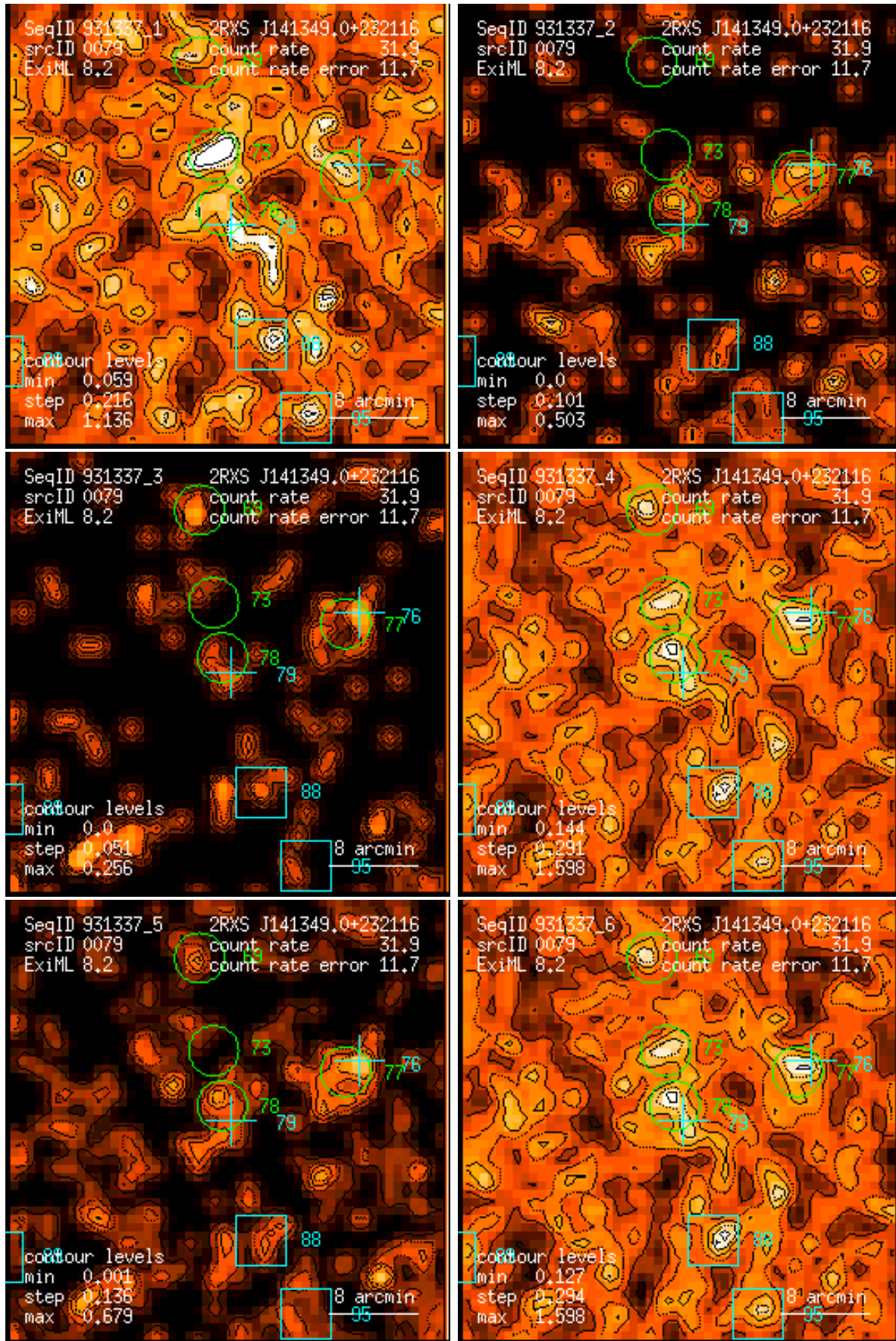
Figure 79: RASS 931337: detection 0079: band rate images, Gaussian filter: (1) PSPC channels 11 – 41, (2) 52 – 90, (3) 91 – 201, (4) 11 – 235, (5) 52 – 201, (6) 11 – 201. Broad band rates in counts/ks. Band rate contour levels in counts/ks/arcmin 2 .
