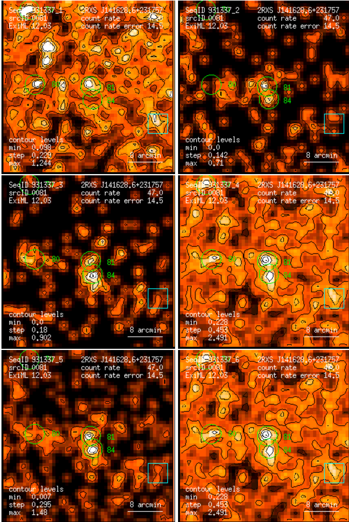
Figure 81: RASS 931337: detection 0081: band rate images, Gaussian filter: (1) PSPC channels 11 – 41, (2) 52 – 90, (3) 91 – 201, (4) 11 – 235, (5) 52 – 201, (6) 11 – 201. Broad band rates in counts/ks. Band rate contour levels in counts/ks/arcmin 2 .
