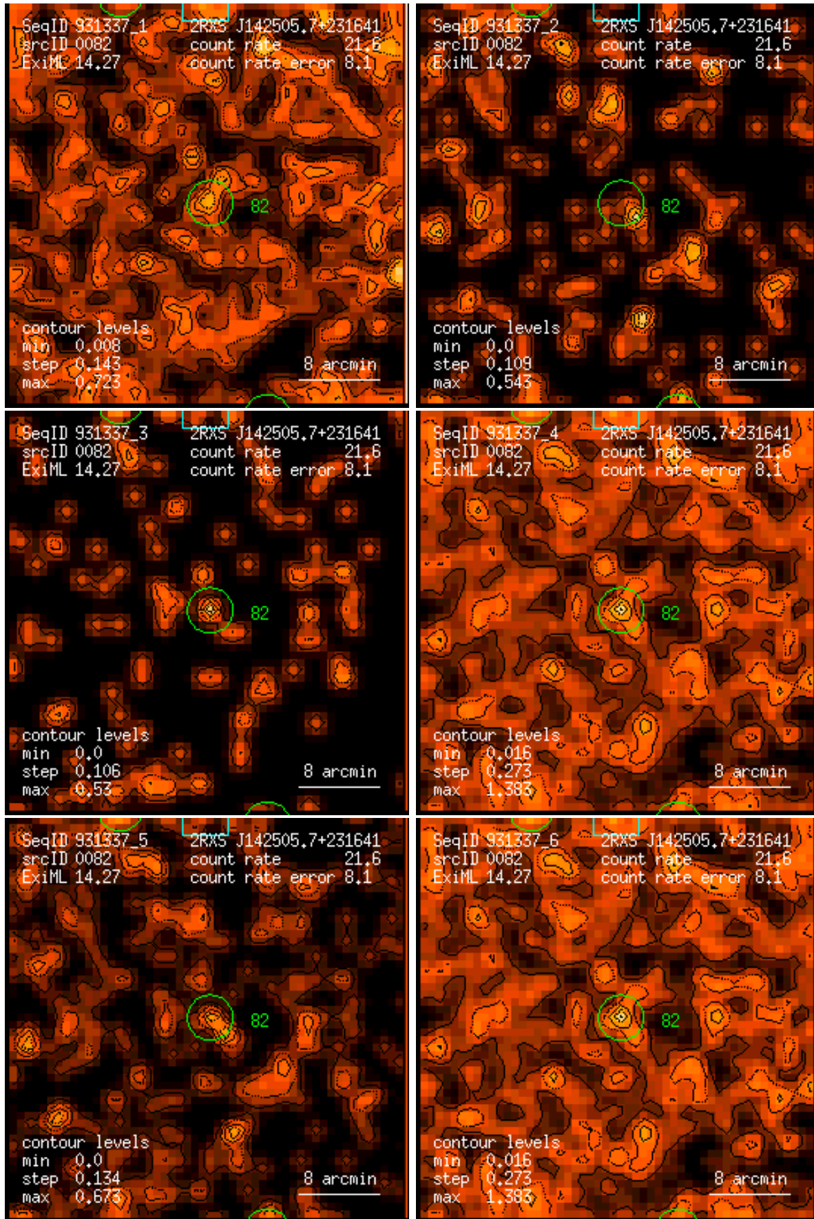
Figure 82: RASS 931337: detection 0082: band rate images, Gaussian filter: (1) PSPC channels 11 – 41, (2) 52 – 90, (3) 91 – 201, (4) 11 – 235, (5) 52 – 201, (6) 11 – 201. Broad band rates in counts/ks. Band rate contour levels in counts/ks/arcmin 2 .
