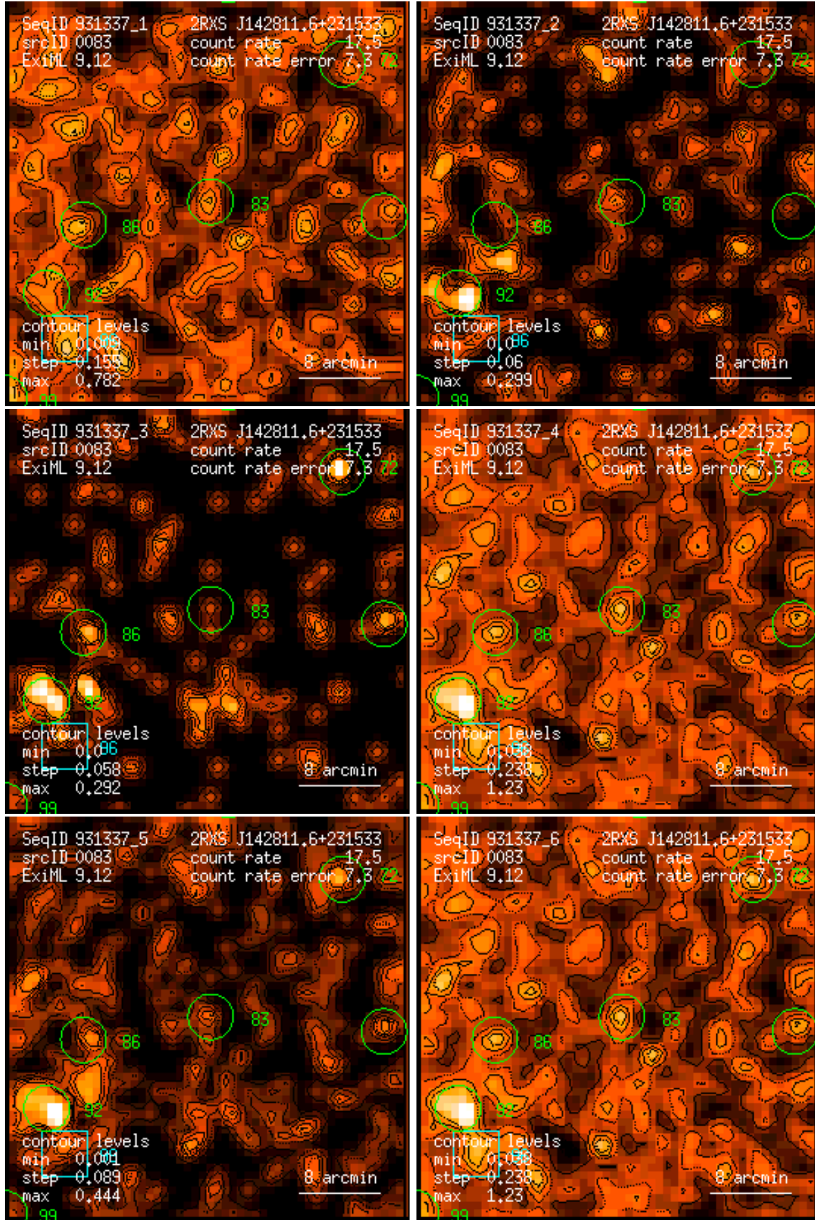
Figure 83: RASS 931337: detection 0083: band rate images, Gaussian filter: (1) PSPC channels 11 – 41, (2) 52 – 90, (3) 91 – 201, (4) 11 – 235, (5) 52 – 201, (6) 11 – 201. Broad band rates in counts/ks. Band rate contour levels in counts/ks/arcmin 2 .
