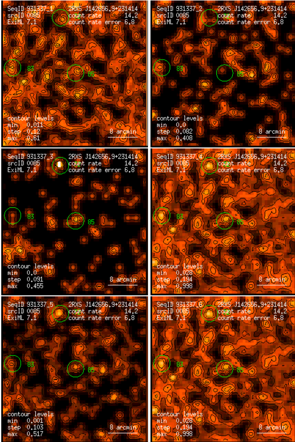
Figure 85: RASS 931337: detection 0085: band rate images, Gaussian filter: (1) PSPC channels 11 – 41, (2) 52 – 90, (3) 91 – 201, (4) 11 – 235, (5) 52 – 201, (6) 11 – 201. Broad band rates in counts/ks. Band rate contour levels in counts/ks/arcmin 2 .
