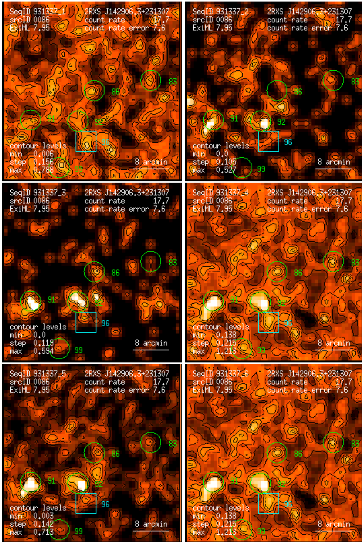
Figure 86: RASS 931337: detection 0086: band rate images, Gaussian filter: (1) PSPC channels 11 – 41, (2) 52 – 90, (3) 91 – 201, (4) 11 – 235, (5) 52 – 201, (6) 11 – 201. Broad band rates in counts/ks. Band rate contour levels in counts/ks/arcmin 2 .
