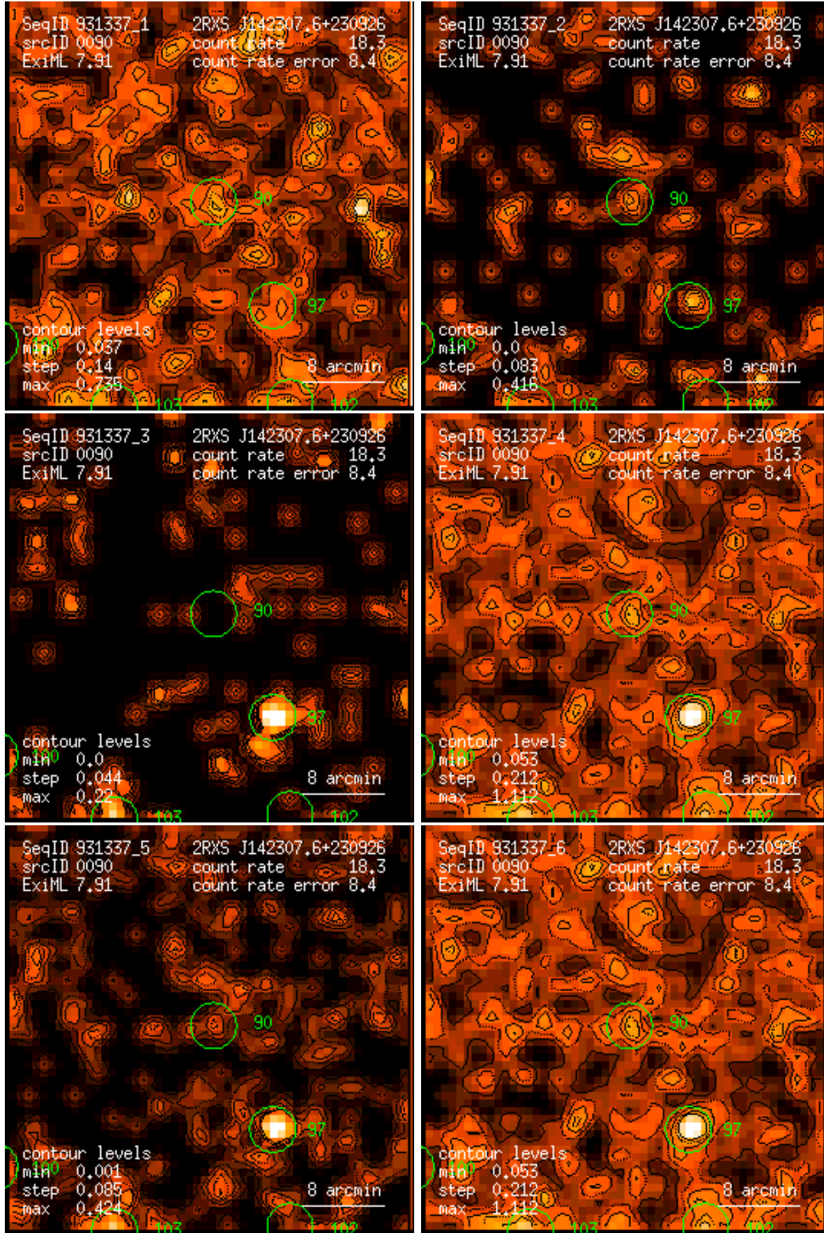
Figure 90: RASS 931337: detection 0090: band rate images, Gaussian filter: (1) PSPC channels 11 – 41, (2) 52 – 90, (3) 91 – 201, (4) 11 – 235, (5) 52 – 201, (6) 11 – 201. Broad band rates in counts/ks. Band rate contour levels in counts/ks/arcmin 2 .
