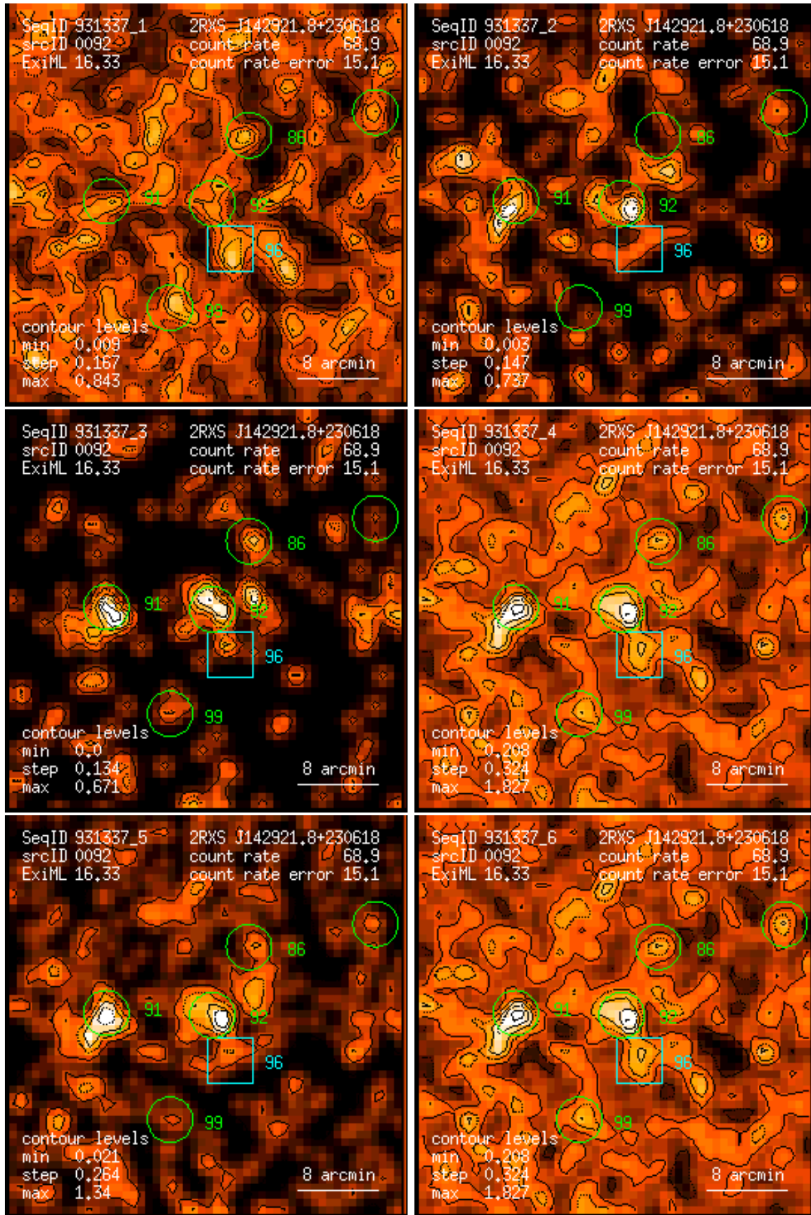
Figure 92: RASS 931337: detection 0092: band rate images, Gaussian filter: (1) PSPC channels 11 – 41, (2) 52 – 90, (3) 91 – 201, (4) 11 – 235, (5) 52 – 201, (6) 11 – 201. Broad band rates in counts/ks. Band rate contour levels in counts/ks/arcmin 2 .
