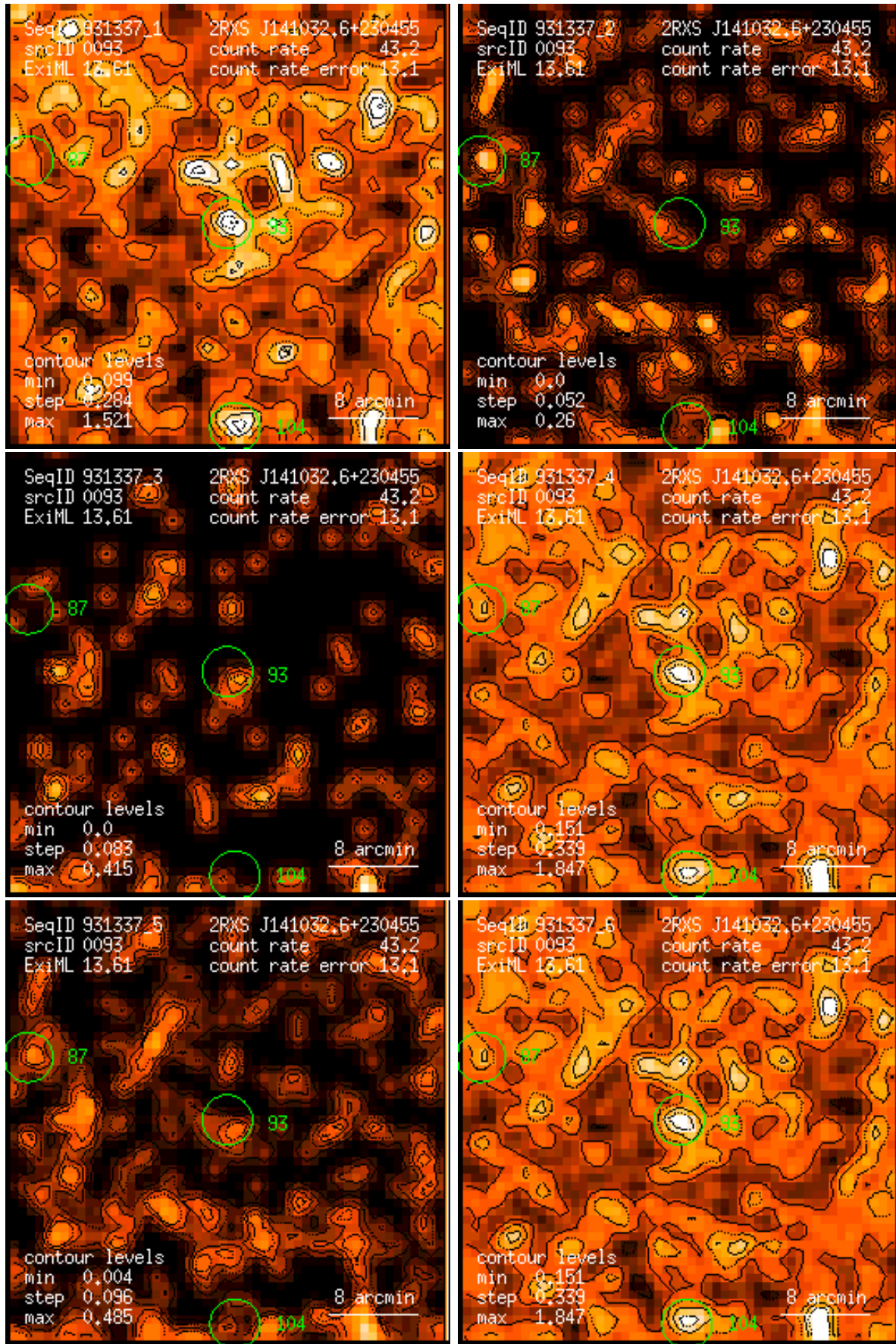
Figure 93: RASS 931337: detection 0093: band rate images, Gaussian filter: (1) PSPC channels 11 – 41, (2) 52 – 90, (3) 91 – 201, (4) 11 – 235, (5) 52 – 201, (6) 11 – 201. Broad band rates in counts/ks. Band rate contour levels in counts/ks/arcmin 2 .
