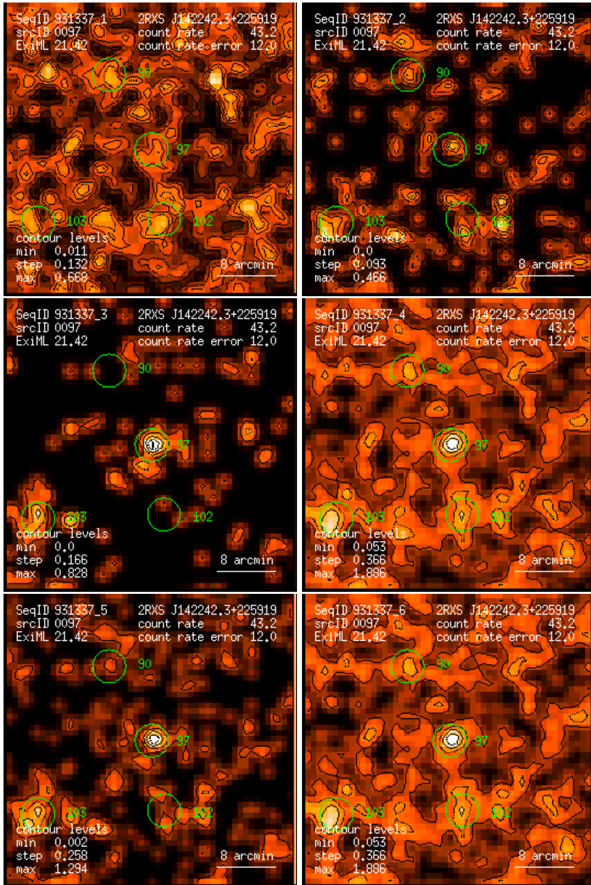
Figure 97: RASS 931337: detection 0097: band rate images, Gaussian filter: (1) PSPC channels 11 – 41, (2) 52 – 90, (3) 91 – 201, (4) 11 – 235, (5) 52 – 201, (6) 11 – 201. Broad band rates in counts/ks. Band rate contour levels in counts/ks/arcmin 2 .
