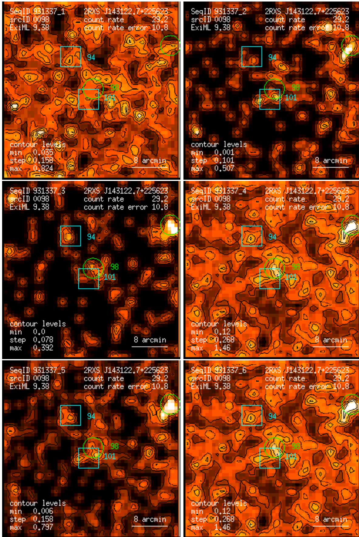
Figure 98: RASS 931337: detection 0098: band rate images, Gaussian filter: (1) PSPC channels 11 – 41, (2) 52 – 90, (3) 91 – 201, (4) 11 – 235, (5) 52 – 201, (6) 11 – 201. Broad band rates in counts/ks. Band rate contour levels in counts/ks/arcmin 2 .
