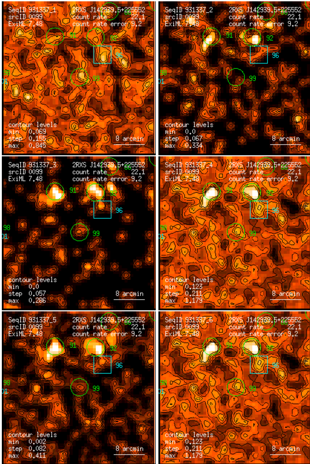
Figure 99: RASS 931337: detection 0099: band rate images, Gaussian filter: (1) PSPC channels 11 – 41, (2) 52 – 90, (3) 91 – 201, (4) 11 – 235, (5) 52 – 201, (6) 11 – 201. Broad band rates in counts/ks. Band rate contour levels in counts/ks/arcmin 2 .
