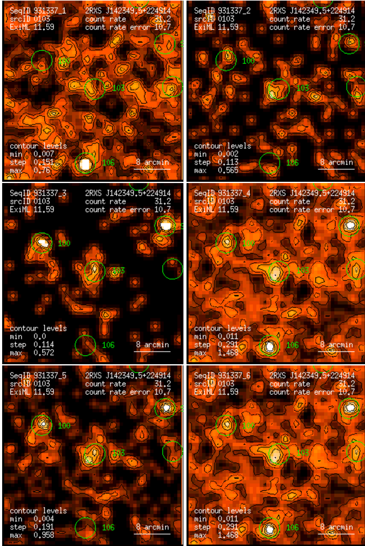
Figure 103: RASS 931337: detection 0103: band rate images, Gaussian filter: (1) PSPC channels 11 – 41, (2) 52 – 90, (3) 91 – 201, (4) 11 – 235, (5) 52 – 201, (6) 11 – 201. Broad band rates in counts/ks. Band rate contour levels in counts/ks/arcmin 2 .
