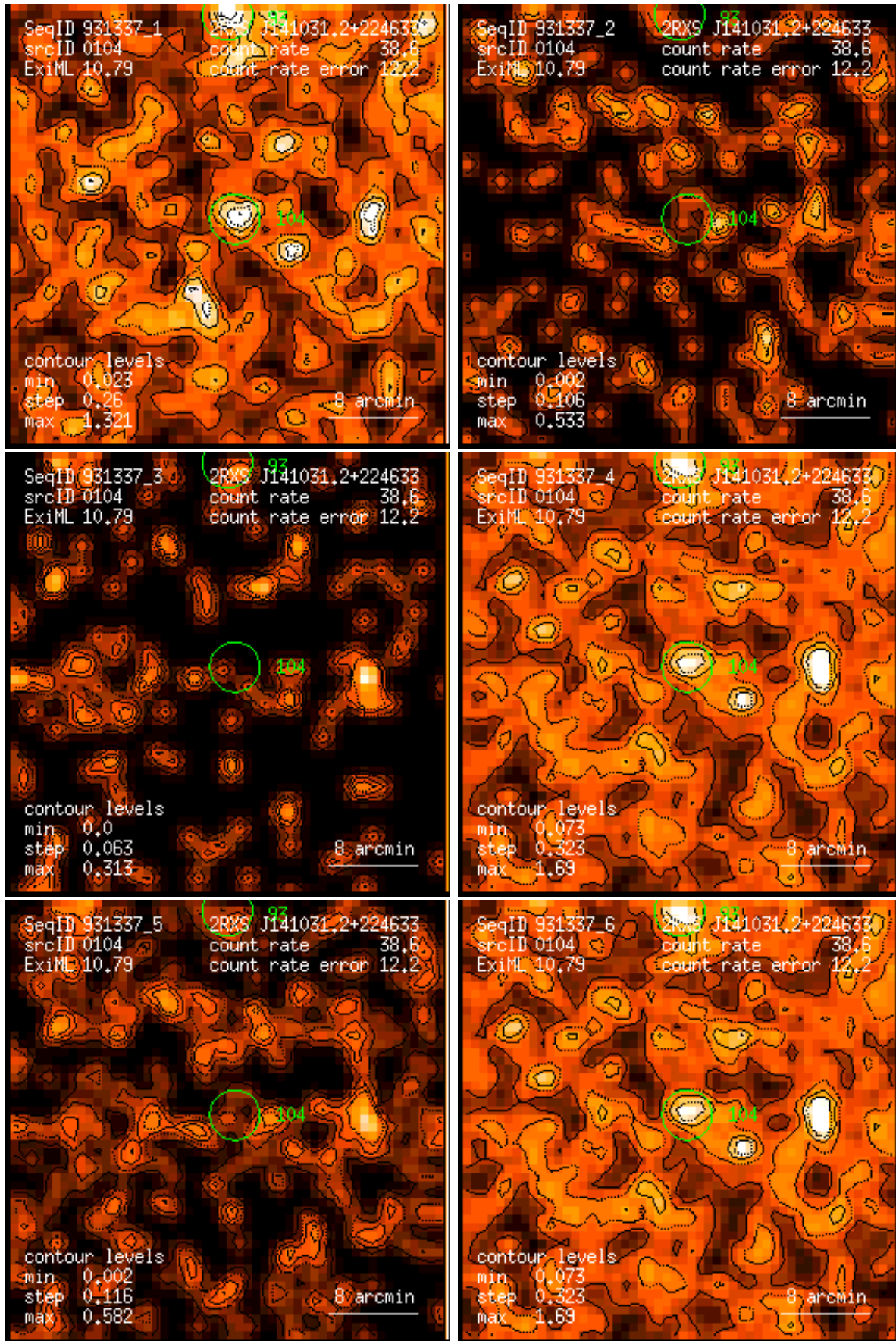
Figure 104: RASS 931337: detection 0104: band rate images, Gaussian filter: (1) PSPC channels 11 – 41, (2) 52 – 90, (3) 91 – 201, (4) 11 – 235, (5) 52 – 201, (6) 11 – 201. Broad band rates in counts/ks. Band rate contour levels in counts/ks/arcmin 2 .
