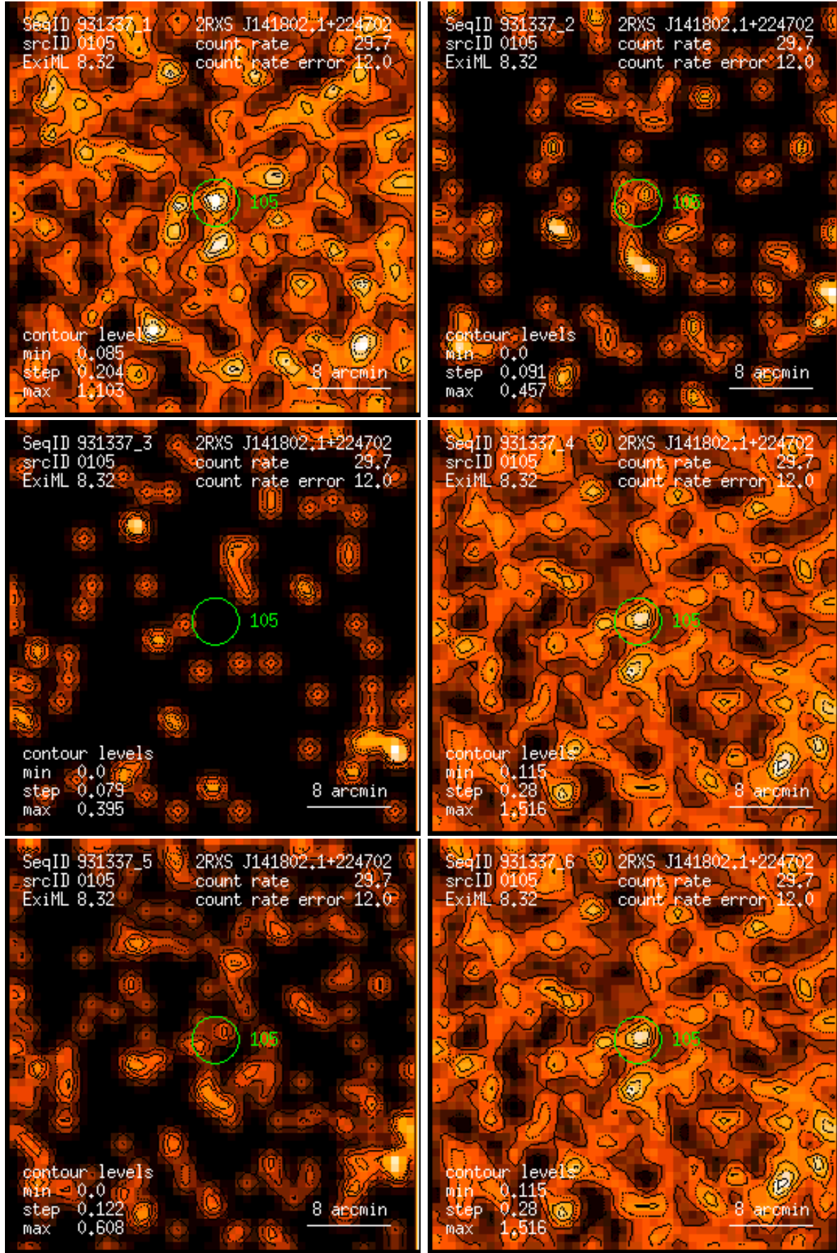
Figure 105: RASS 931337: detection 0105: band rate images, Gaussian filter: (1) PSPC channels 11 – 41, (2) 52 – 90, (3) 91 – 201, (4) 11 – 235, (5) 52 – 201, (6) 11 – 201. Broad band rates in counts/ks. Band rate contour levels in counts/ks/arcmin 2 .
