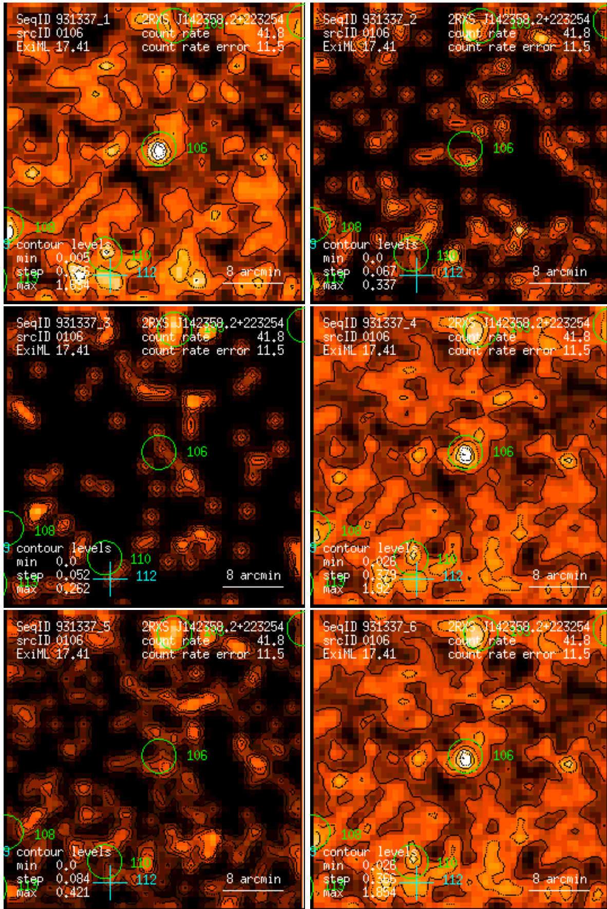
Figure 106: RASS 931337: detection 0106: band rate images, Gaussian filter: (1) PSPC channels 11 – 41, (2) 52 – 90, (3) 91 – 201, (4) 11 – 235, (5) 52 – 201, (6) 11 – 201. Broad band rates in counts/ks. Band rate contour levels in counts/ks/arcmin 2 .
