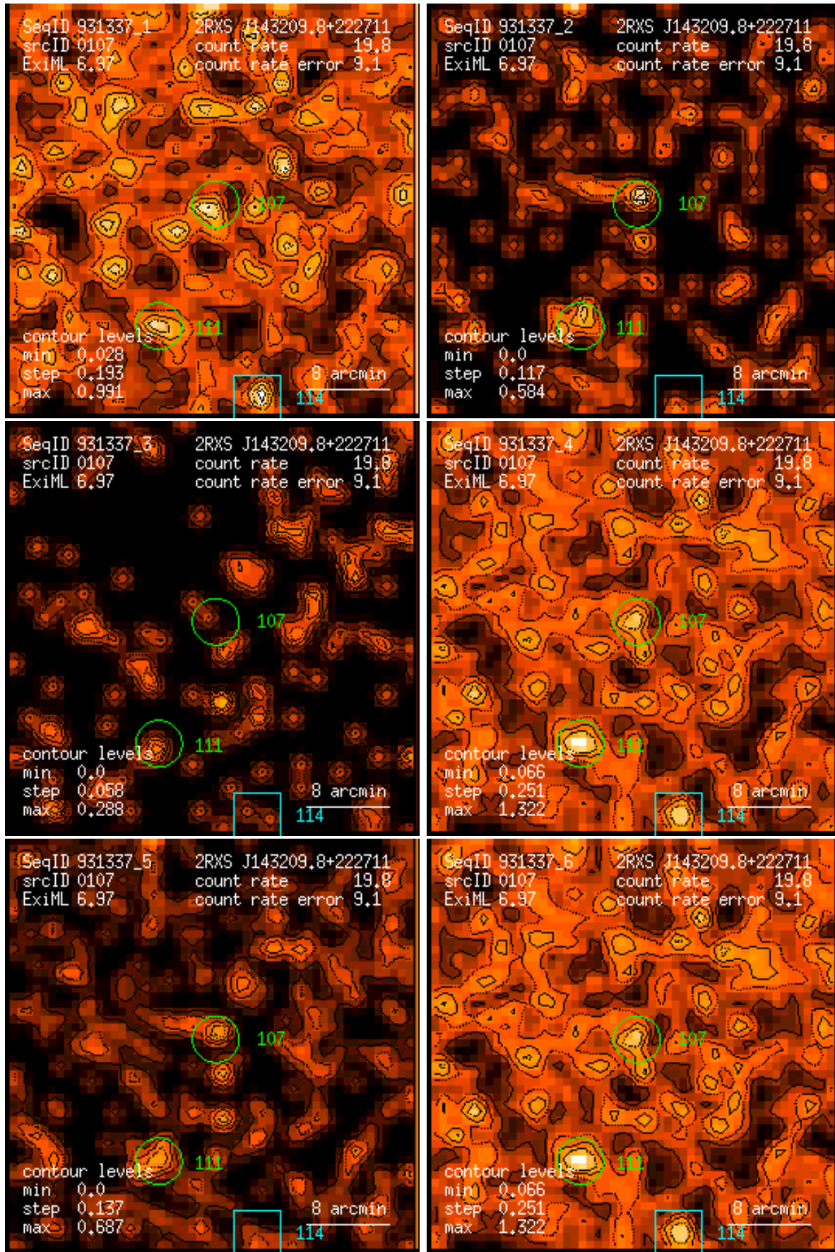
Figure 107: RASS 931337: detection 0107: band rate images, Gaussian filter: (1) PSPC channels 11 – 41, (2) 52 – 90, (3) 91 – 201, (4) 11 – 235, (5) 52 – 201, (6) 11 – 201. Broad band rates in counts/ks. Band rate contour levels in counts/ks/arcmin 2 .
