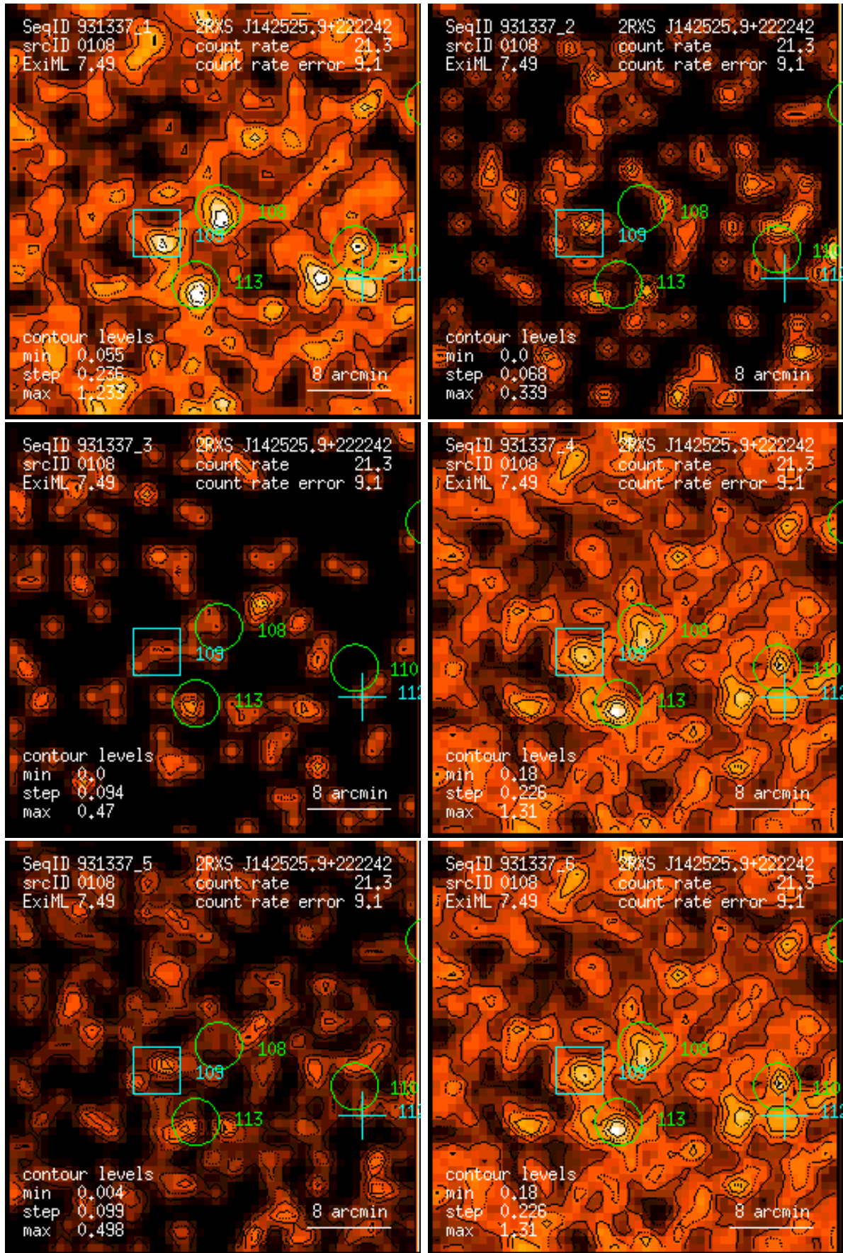
Figure 108: RASS 931337: detection 0108: band rate images, Gaussian filter: (1) PSPC channels 11 – 41, (2) 52 – 90, (3) 91 – 201, (4) 11 – 235, (5) 52 – 201, (6) 11 – 201. Broad band rates in counts/ks. Band rate contour levels in counts/ks/arcmin 2 .
