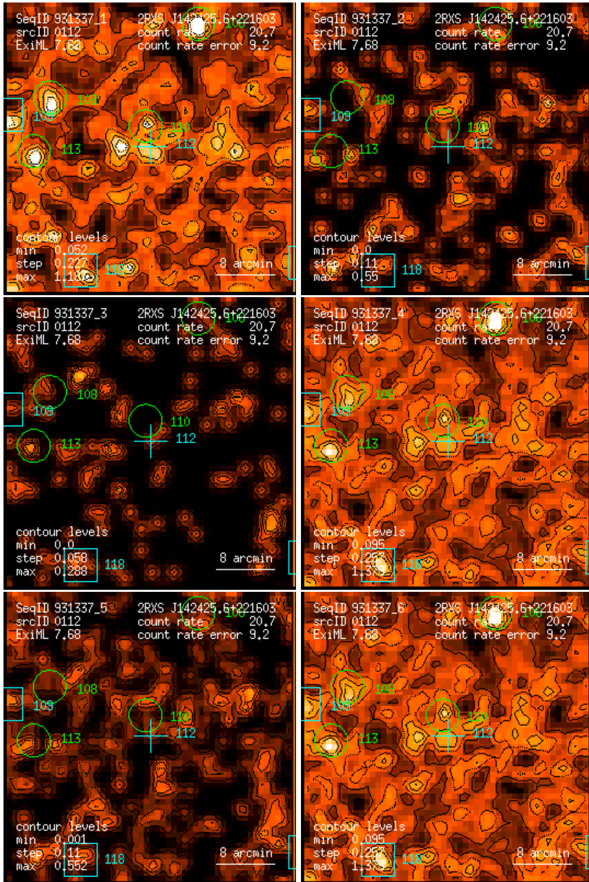
Figure 112: RASS 931337: detection 0112: band rate images, Gaussian filter: (1) PSPC channels 11 – 41, (2) 52 – 90, (3) 91 – 201, (4) 11 – 235, (5) 52 – 201, (6) 11 – 201. Broad band rates in counts/ks. Band rate contour levels in counts/ks/arcmin 2 .
