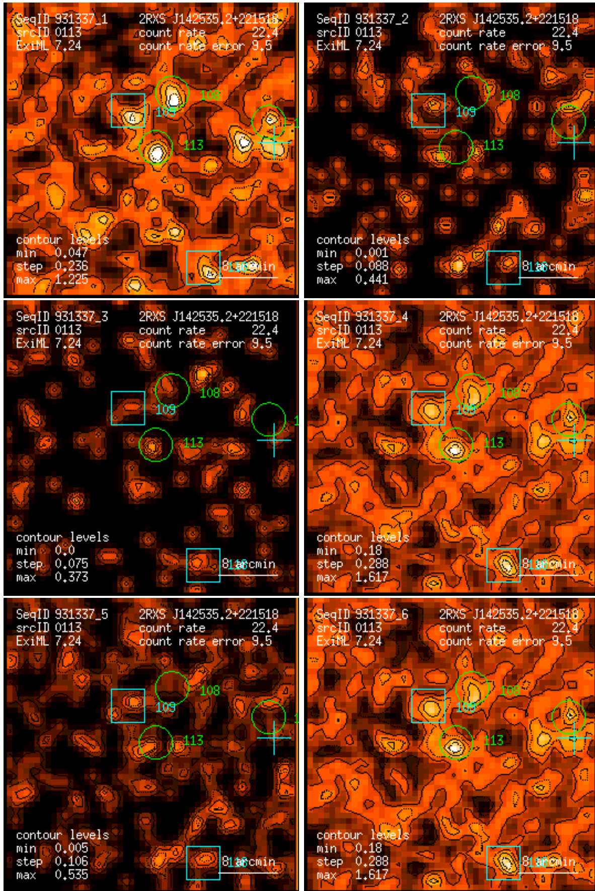
Figure 113: RASS 931337: detection 0113: band rate images, Gaussian filter: (1) PSPC channels 11 – 41, (2) 52 – 90, (3) 91 – 201, (4) 11 – 235, (5) 52 – 201, (6) 11 – 201. Broad band rates in counts/ks. Band rate contour levels in counts/ks/arcmin 2 .
