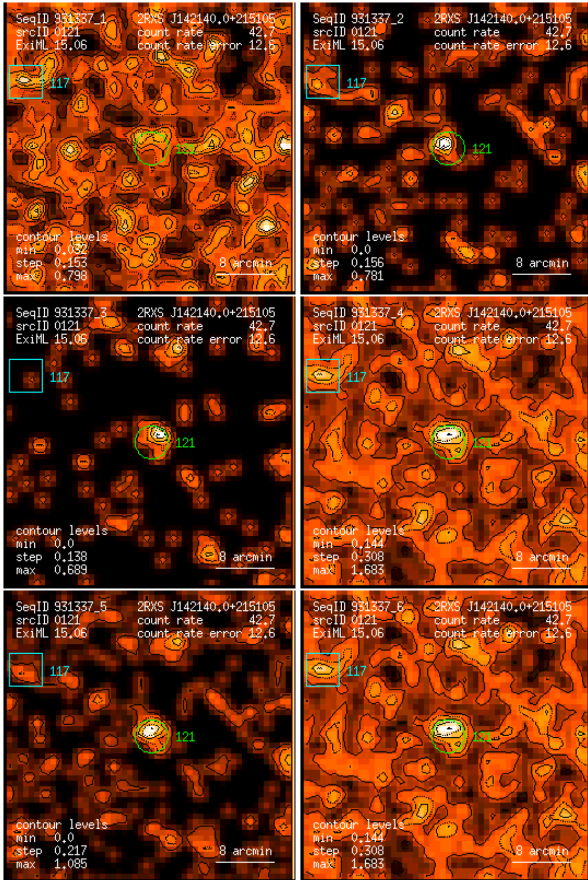
Figure 121: RASS 931337: detection 0121: band rate images, Gaussian filter: (1) PSPC channels 11 – 41, (2) 52 – 90, (3) 91 – 201, (4) 11 – 235, (5) 52 – 201, (6) 11 – 201. Broad band rates in counts/ks. Band rate contour levels in counts/ks/arcmin 2 .
