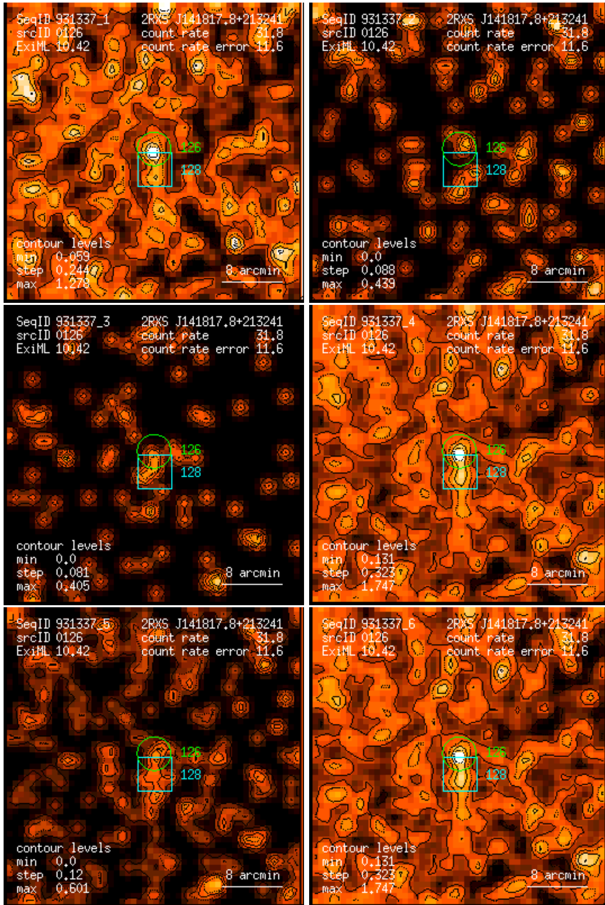
Figure 126: RASS 931337: detection 0126: band rate images, Gaussian filter: (1) PSPC channels 11 – 41, (2) 52 – 90, (3) 91 – 201, (4) 11 – 235, (5) 52 – 201, (6) 11 – 201. Broad band rates in counts/ks. Band rate contour levels in counts/ks/arcmin 2 .
