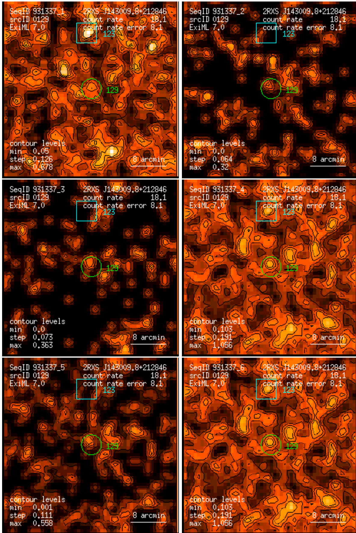
Figure 129: RASS 931337: detection 0129: band rate images, Gaussian filter: (1) PSPC channels 11 – 41, (2) 52 – 90, (3) 91 – 201, (4) 11 – 235, (5) 52 – 201, (6) 11 – 201. Broad band rates in counts/ks. Band rate contour levels in counts/ks/arcmin 2 .
