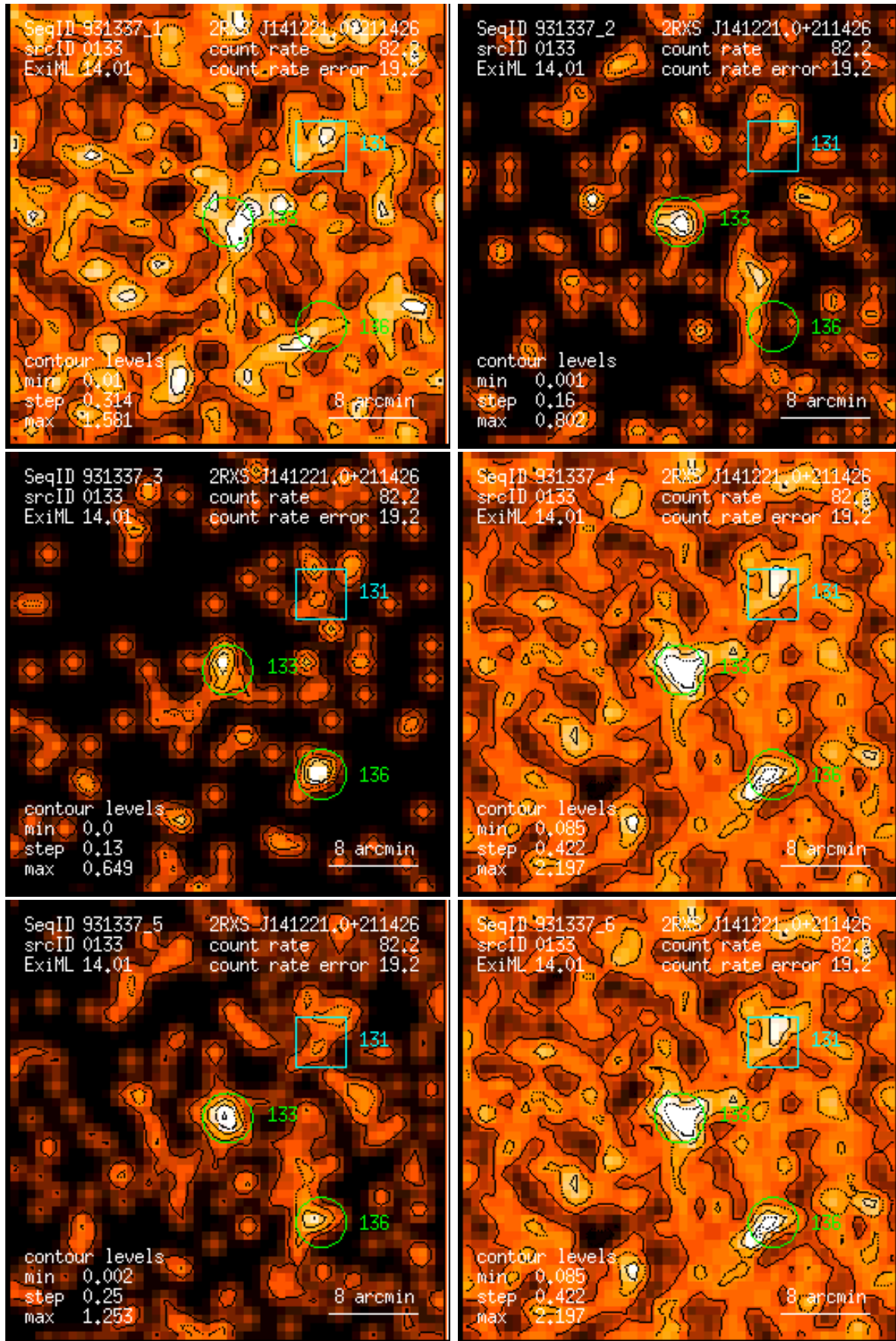
Figure 133: RASS 931337: detection 0133: band rate images, Gaussian filter: (1) PSPC channels 11 – 41, (2) 52 – 90, (3) 91 – 201, (4) 11 – 235, (5) 52 – 201, (6) 11 – 201. Broad band rates in counts/ks. Band rate contour levels in counts/ks/arcmin 2 .
