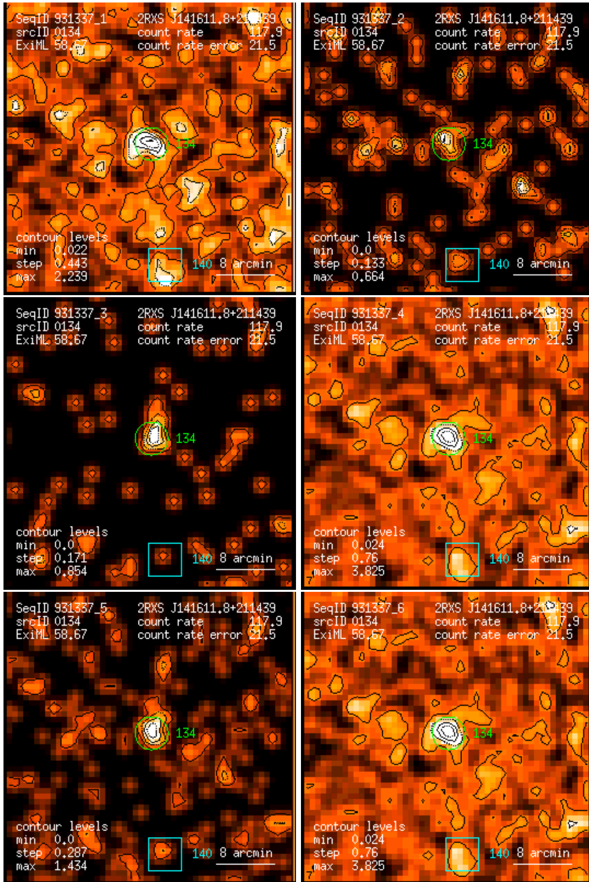
Figure 134: RASS 931337: detection 0134: band rate images, Gaussian filter: (1) PSPC channels 11 – 41, (2) 52 – 90, (3) 91 – 201, (4) 11 – 235, (5) 52 – 201, (6) 11 – 201. Broad band rates in counts/ks. Band rate contour levels in counts/ks/arcmin 2 .
