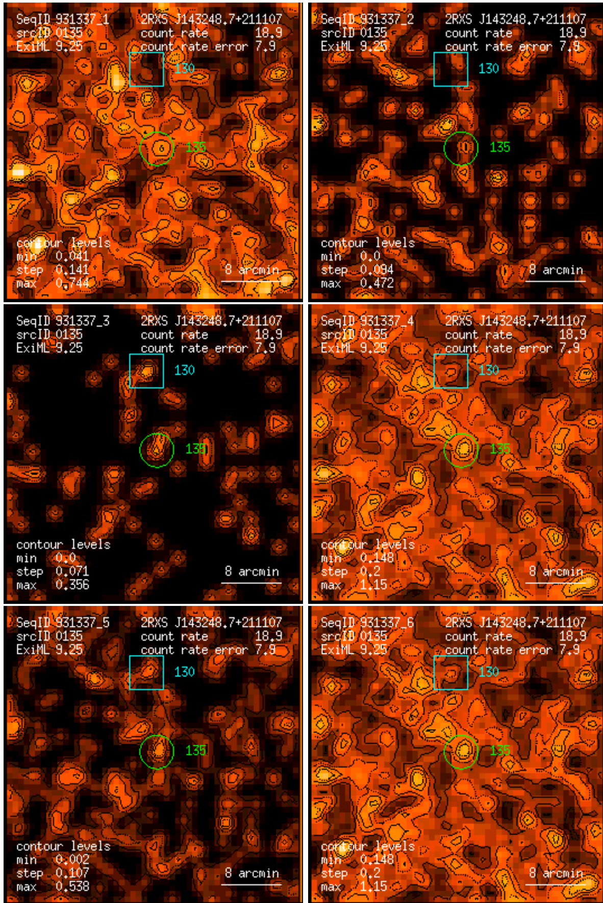
Figure 135: RASS 931337: detection 0135: band rate images, Gaussian filter: (1) PSPC channels 11 – 41, (2) 52 – 90, (3) 91 – 201, (4) 11 – 235, (5) 52 – 201, (6) 11 – 201. Broad band rates in counts/ks. Band rate contour levels in counts/ks/arcmin 2 .
