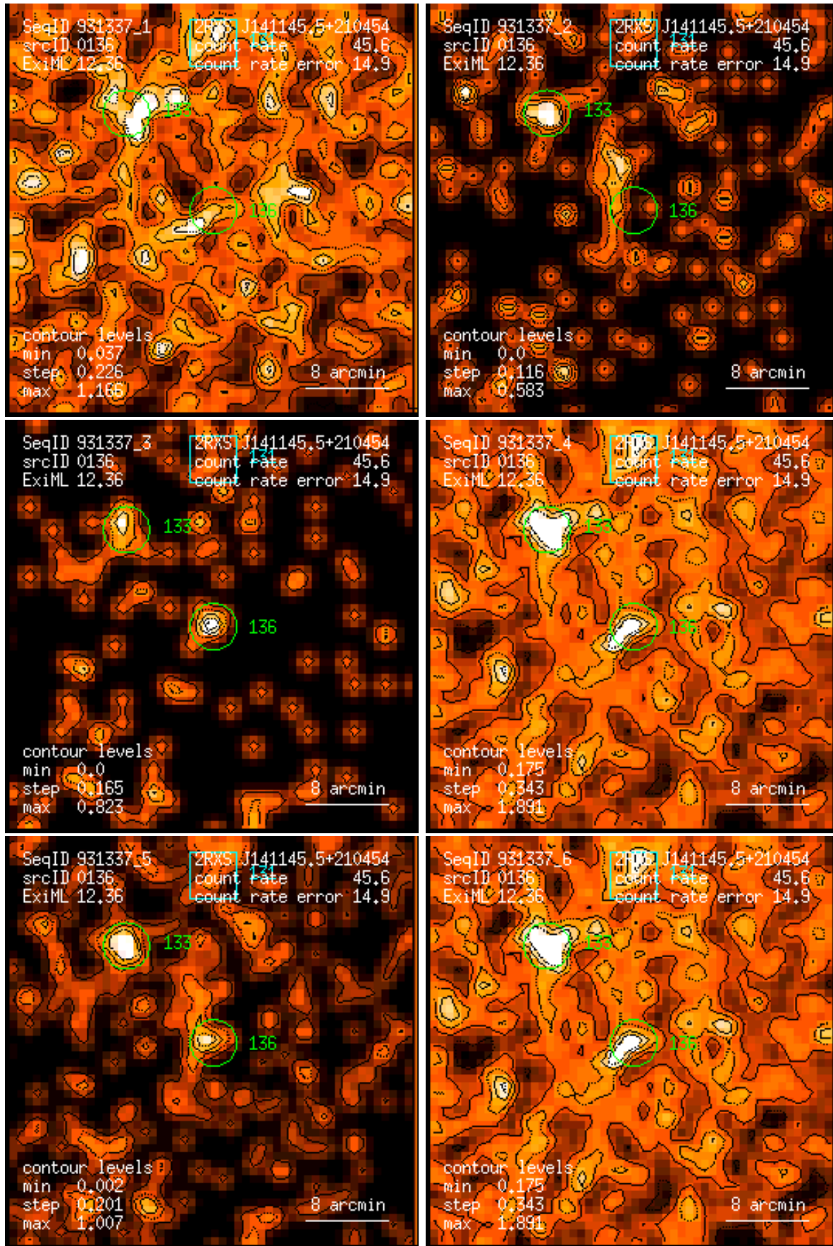
Figure 136: RASS 931337: detection 0136: band rate images, Gaussian filter: (1) PSPC channels 11 – 41, (2) 52 – 90, (3) 91 – 201, (4) 11 – 235, (5) 52 – 201, (6) 11 – 201. Broad band rates in counts/ks. Band rate contour levels in counts/ks/arcmin 2 .
