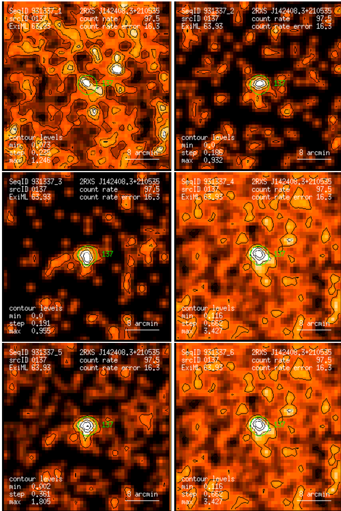
Figure 137: RASS 931337: detection 0137: band rate images, Gaussian filter: (1) PSPC channels 11 – 41, (2) 52 – 90, (3) 91 – 201, (4) 11 – 235, (5) 52 – 201, (6) 11 – 201. Broad band rates in counts/ks. Band rate contour levels in counts/ks/arcmin 2 .
