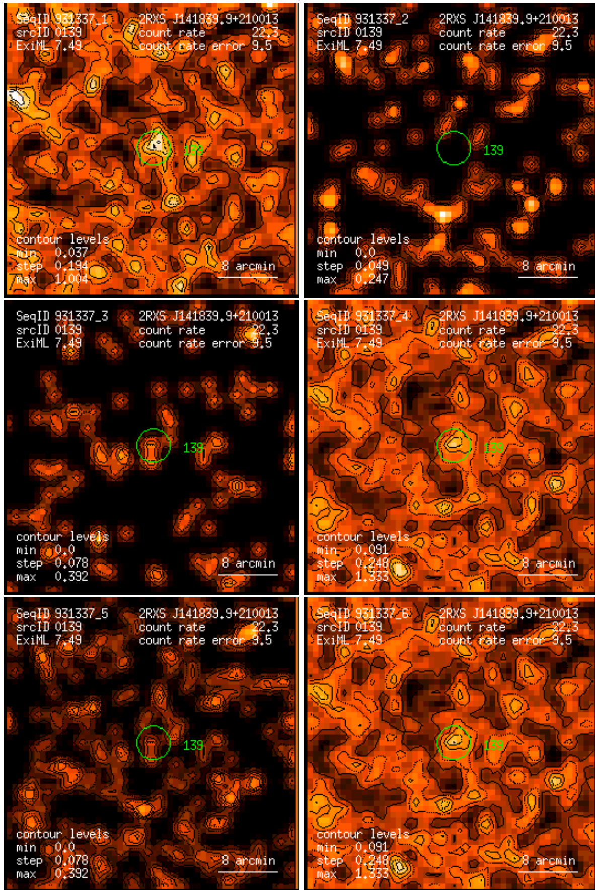
Figure 139: RASS 931337: detection 0139: band rate images, Gaussian filter: (1) PSPC channels 11 – 41, (2) 52 – 90, (3) 91 – 201, (4) 11 – 235, (5) 52 – 201, (6) 11 – 201. Broad band rates in counts/ks. Band rate contour levels in counts/ks/arcmin 2 .
