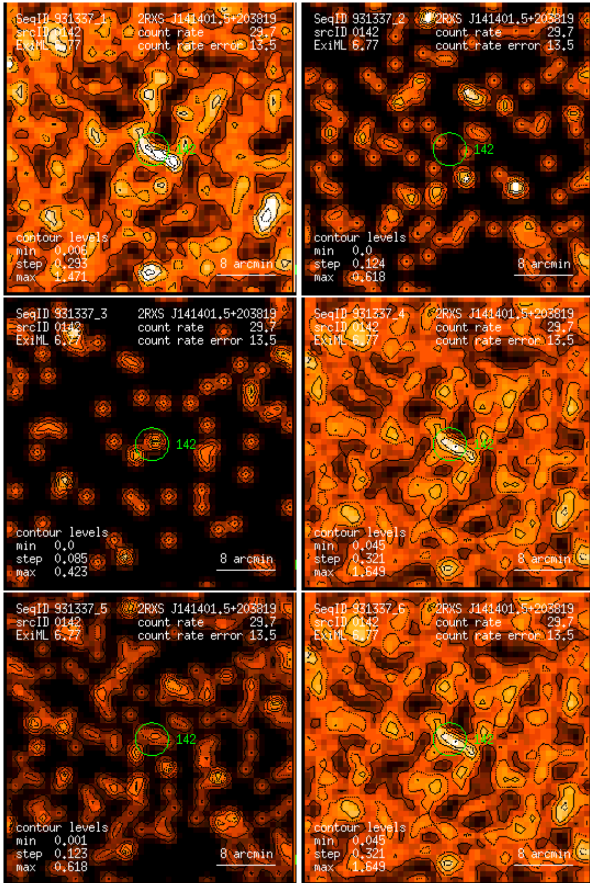
Figure 142: RASS 931337: detection 0142: band rate images, Gaussian filter: (1) PSPC channels 11 – 41, (2) 52 – 90, (3) 91 – 201, (4) 11 – 235, (5) 52 – 201, (6) 11 – 201. Broad band rates in counts/ks. Band rate contour levels in counts/ks/arcmin 2 .
