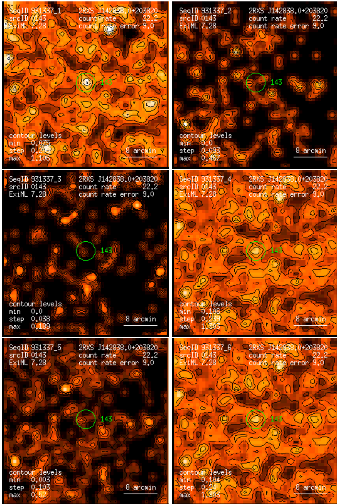
Figure 143: RASS 931337: detection 0143: band rate images, Gaussian filter: (1) PSPC channels 11 – 41, (2) 52 – 90, (3) 91 – 201, (4) 11 – 235, (5) 52 – 201, (6) 11 – 201. Broad band rates in counts/ks. Band rate contour levels in counts/ks/arcmin 2 .
