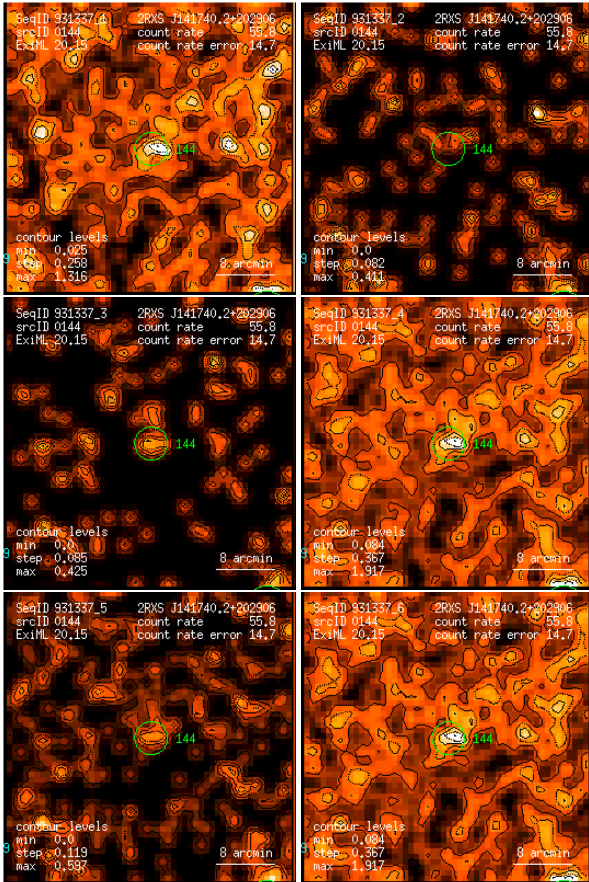
Figure 144: RASS 931337: detection 0144: band rate images, Gaussian filter: (1) PSPC channels 11 – 41, (2) 52 – 90, (3) 91 – 201, (4) 11 – 235, (5) 52 – 201, (6) 11 – 201. Broad band rates in counts/ks. Band rate contour levels in counts/ks/arcmin 2 .
