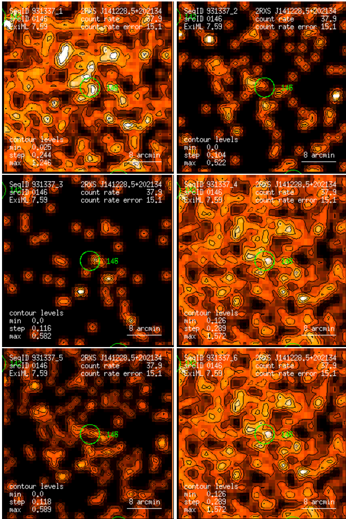
Figure 146: RASS 931337: detection 0146: band rate images, Gaussian filter: (1) PSPC channels 11 – 41, (2) 52 – 90, (3) 91 – 201, (4) 11 – 235, (5) 52 – 201, (6) 11 – 201. Broad band rates in counts/ks. Band rate contour levels in counts/ks/arcmin 2 .
