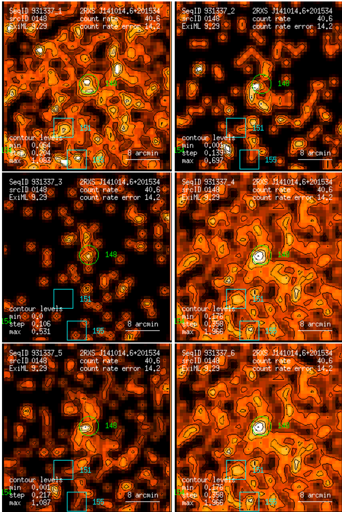
Figure 148: RASS 931337: detection 0148: band rate images, Gaussian filter: (1) PSPC channels 11 – 41, (2) 52 – 90, (3) 91 – 201, (4) 11 – 235, (5) 52 – 201, (6) 11 – 201. Broad band rates in counts/ks. Band rate contour levels in counts/ks/arcmin 2 .
