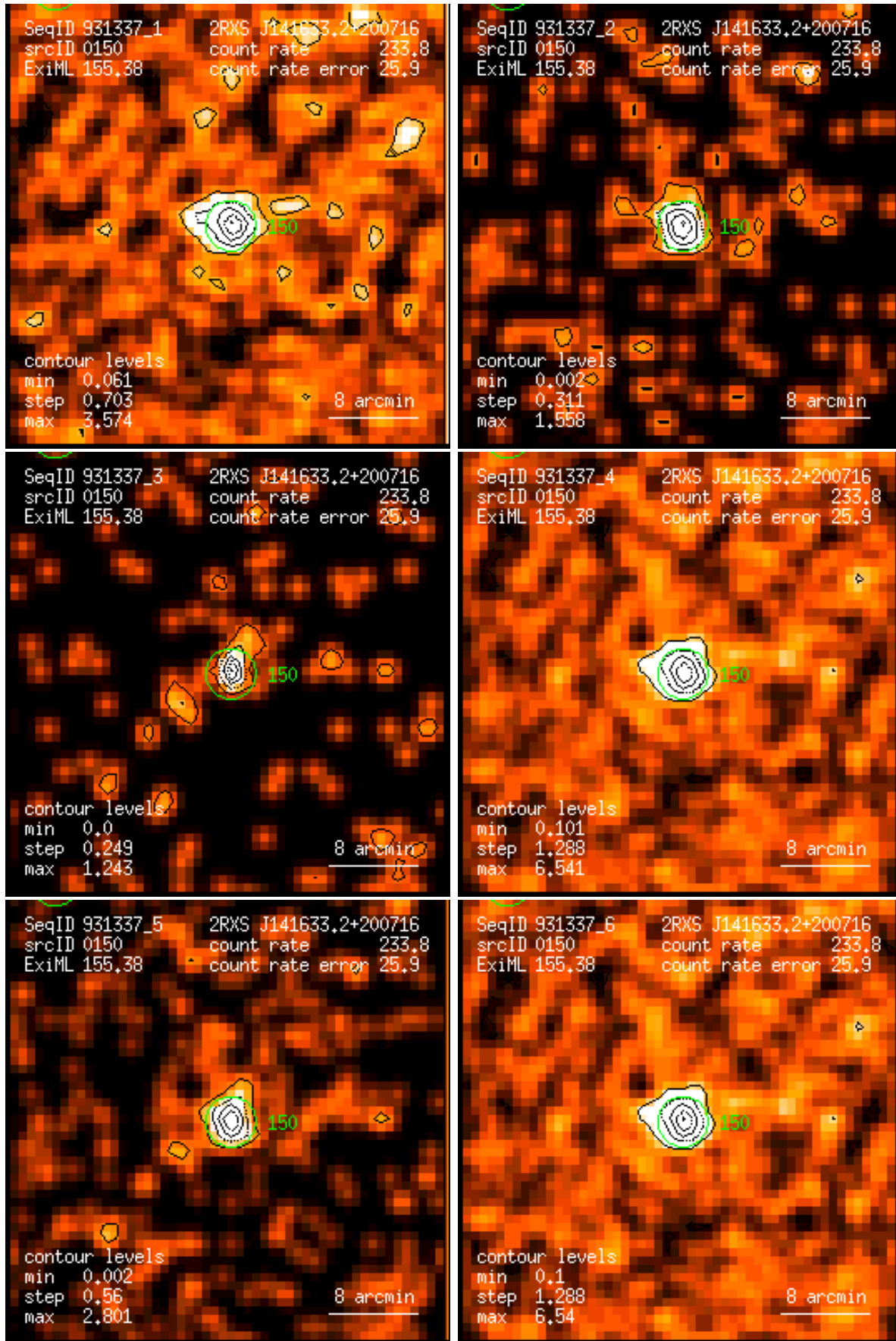
Figure 150: RASS 931337: detection 0150: band rate images, Gaussian filter: (1) PSPC channels 11 – 41, (2) 52 – 90, (3) 91 – 201, (4) 11 – 235, (5) 52 – 201, (6) 11 – 201. Broad band rates in counts/ks. Band rate contour levels in counts/ks/arcmin 2 .
