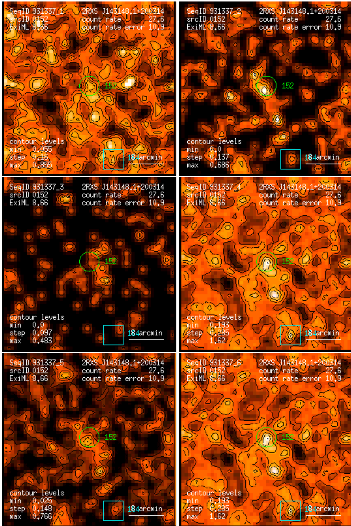
Figure 152: RASS 931337: detection 0152: band rate images, Gaussian filter: (1) PSPC channels 11 – 41, (2) 52 – 90, (3) 91 – 201, (4) 11 – 235, (5) 52 – 201, (6) 11 – 201. Broad band rates in counts/ks. Band rate contour levels in counts/ks/arcmin 2 .
