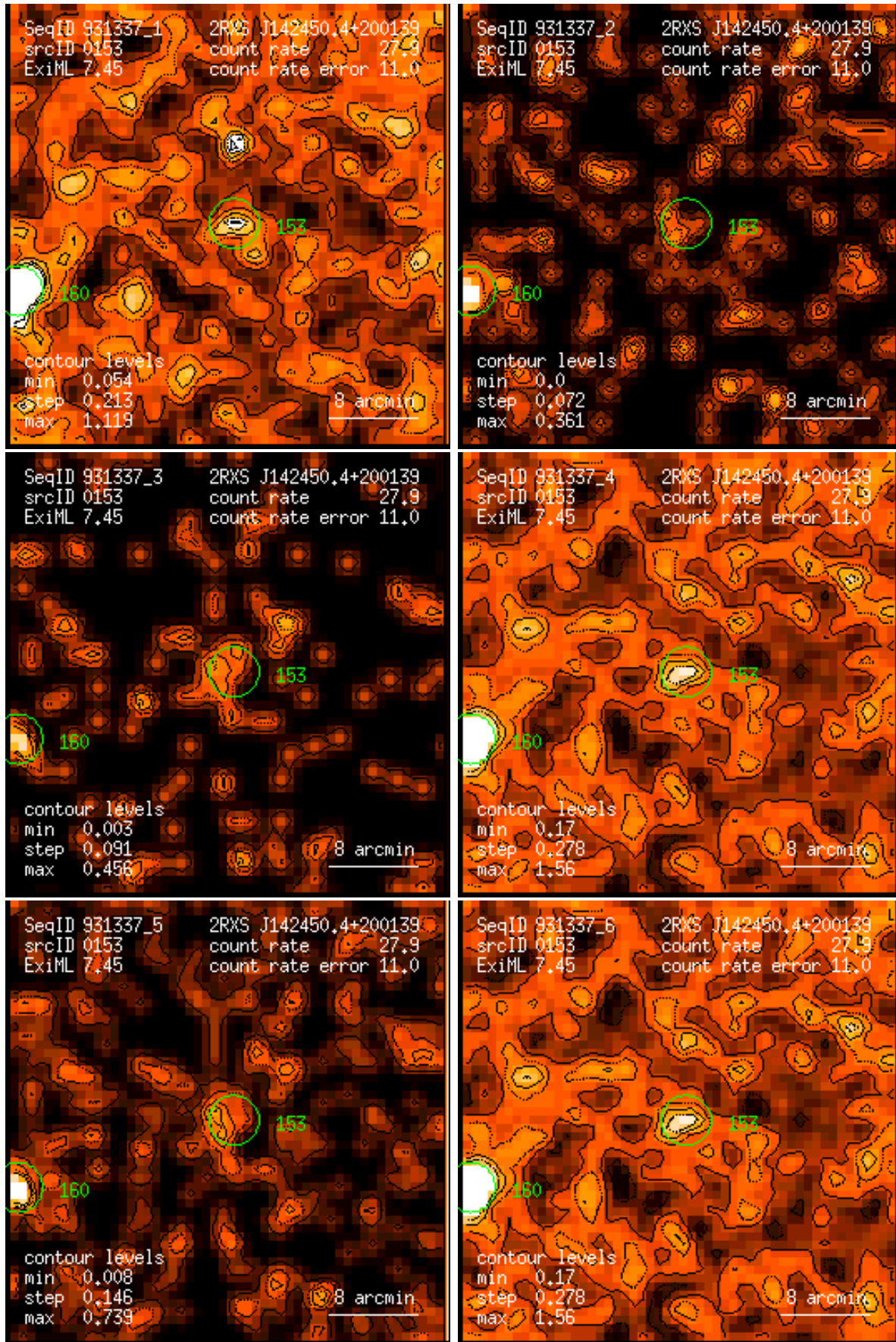
Figure 153: RASS 931337: detection 0153: band rate images, Gaussian filter: (1) PSPC channels 11 – 41, (2) 52 – 90, (3) 91 – 201, (4) 11 – 235, (5) 52 – 201, (6) 11 – 201. Broad band rates in counts/ks. Band rate contour levels in counts/ks/arcmin 2 .
