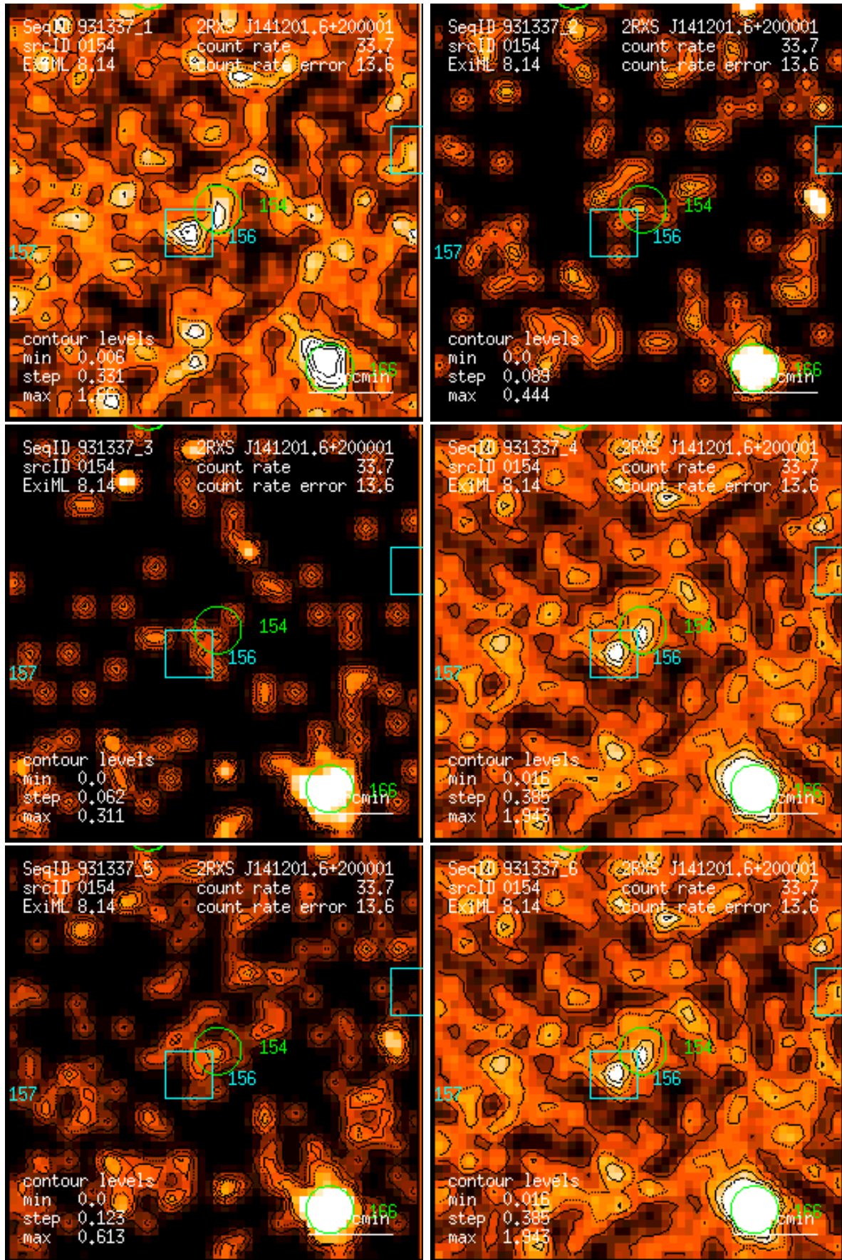
Figure 154: RASS 931337: detection 0154: band rate images, Gaussian filter: (1) PSPC channels 11 – 41, (2) 52 – 90, (3) 91 – 201, (4) 11 – 235, (5) 52 – 201, (6) 11 – 201. Broad band rates in counts/ks. Band rate contour levels in counts/ks/arcmin 2 .
