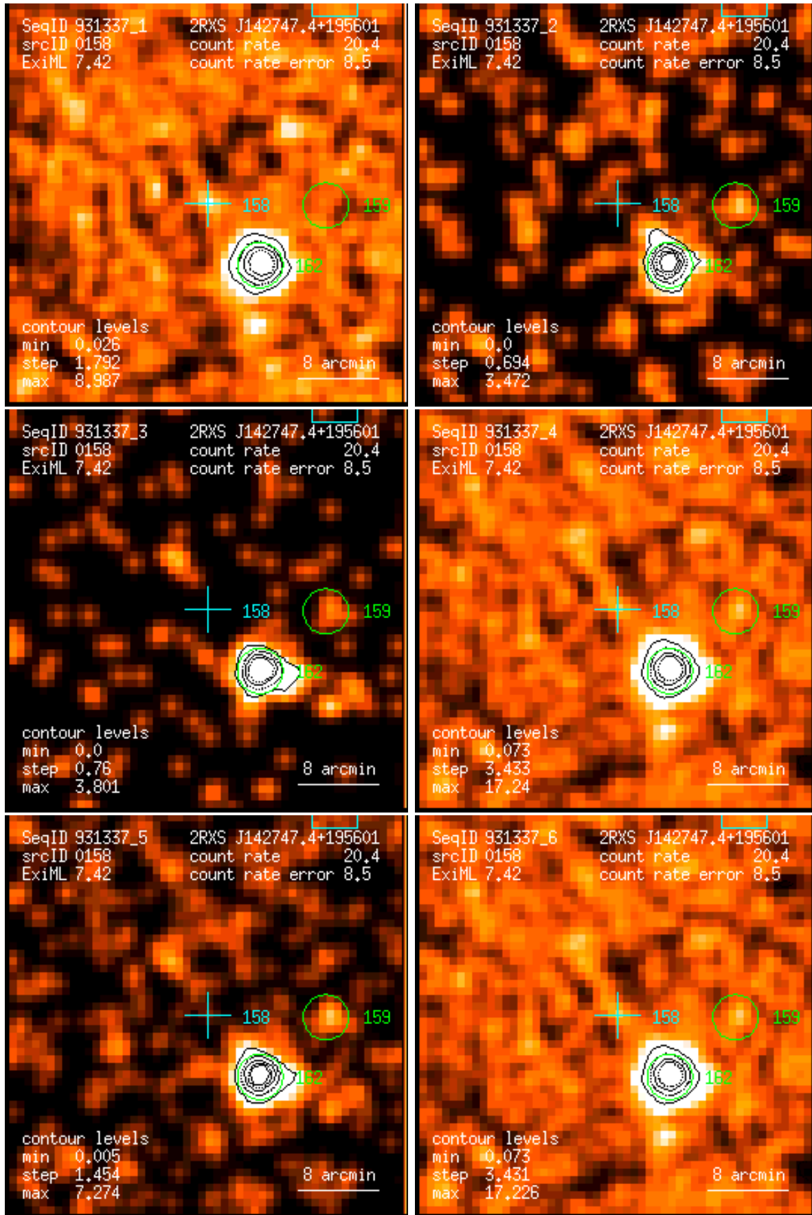
Figure 158: RASS 931337: detection 0158: band rate images, Gaussian filter: (1) PSPC channels 11 – 41, (2) 52 – 90, (3) 91 – 201, (4) 11 – 235, (5) 52 – 201, (6) 11 – 201. Broad band rates in counts/ks. Band rate contour levels in counts/ks/arcmin 2 .
