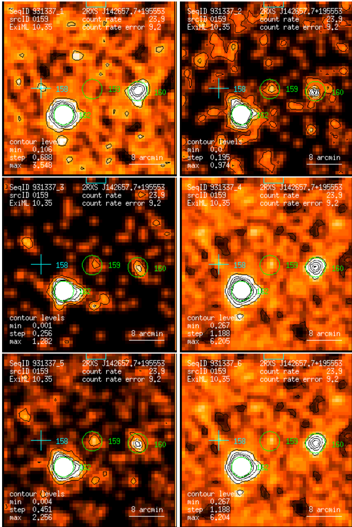
Figure 159: RASS 931337: detection 0159: band rate images, Gaussian filter: (1) PSPC channels 11 – 41, (2) 52 – 90, (3) 91 – 201, (4) 11 – 235, (5) 52 – 201, (6) 11 – 201. Broad band rates in counts/ks. Band rate contour levels in counts/ks/arcmin 2 .
