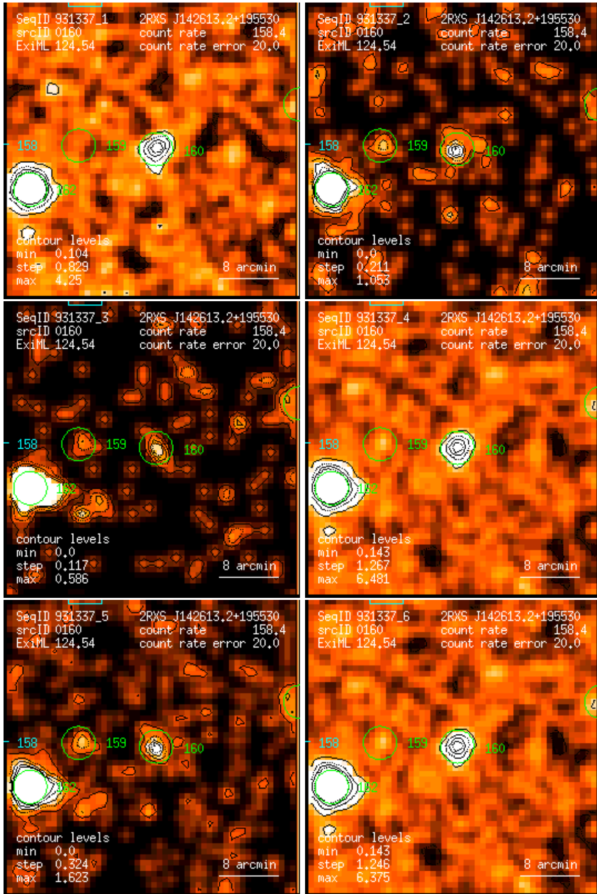
Figure 160: RASS 931337: detection 0160: band rate images, Gaussian filter: (1) PSPC channels 11 – 41, (2) 52 – 90, (3) 91 – 201, (4) 11 – 235, (5) 52 – 201, (6) 11 – 201. Broad band rates in counts/ks. Band rate contour levels in counts/ks/arcmin 2 .
