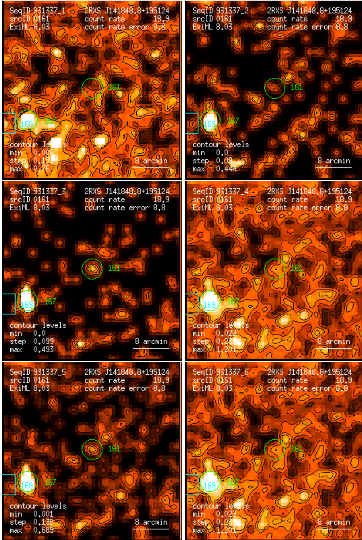
Figure 161: RASS 931337: detection 0161: band rate images, Gaussian filter: (1) PSPC channels 11 – 41, (2) 52 – 90, (3) 91 – 201, (4) 11 – 235, (5) 52 – 201, (6) 11 – 201. Broad band rates in counts/ks. Band rate contour levels in counts/ks/arcmin 2 .
