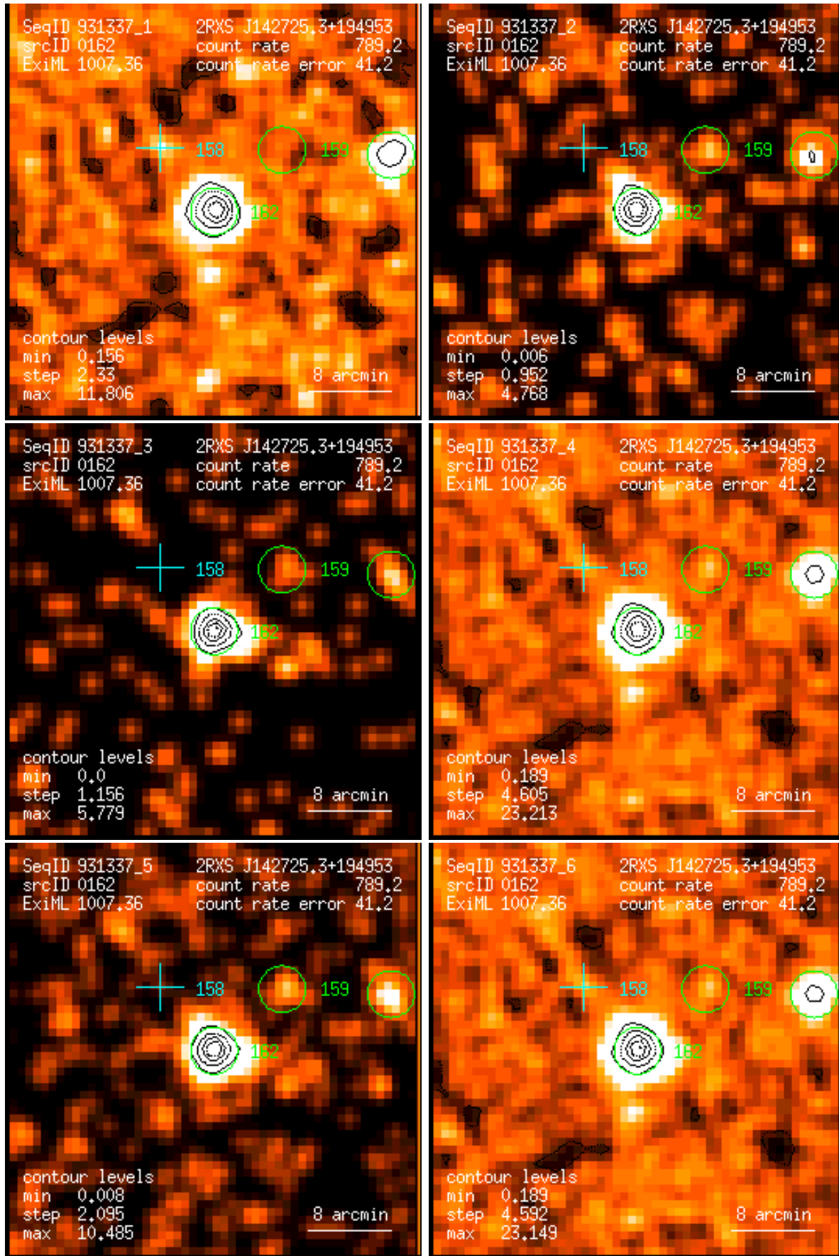
Figure 162: RASS 931337: detection 0162: band rate images, Gaussian filter: (1) PSPC channels 11 – 41, (2) 52 – 90, (3) 91 – 201, (4) 11 – 235, (5) 52 – 201, (6) 11 – 201. Broad band rates in counts/ks. Band rate contour levels in counts/ks/arcmin 2 .
