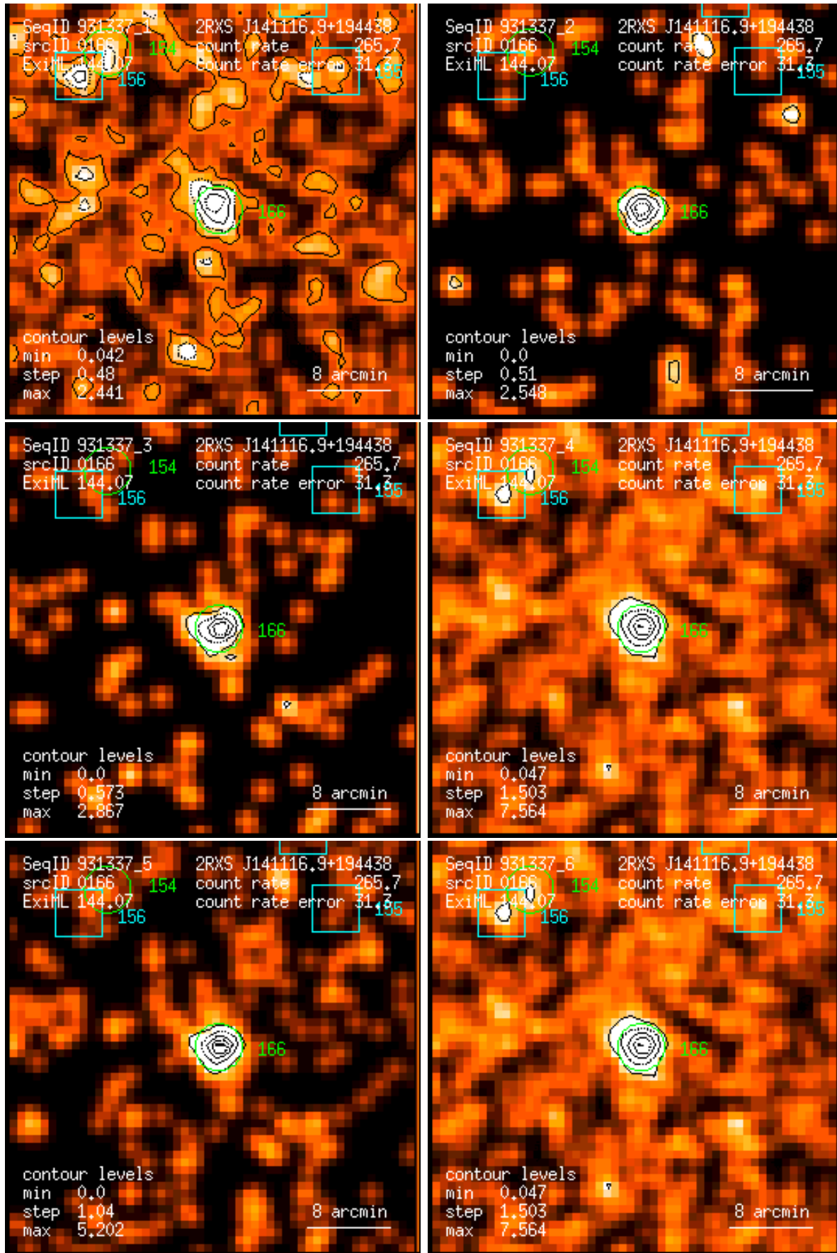
Figure 166: RASS 931337: detection 0166: band rate images, Gaussian filter: (1) PSPC channels 11 – 41, (2) 52 – 90, (3) 91 – 201, (4) 11 – 235, (5) 52 – 201, (6) 11 – 201. Broad band rates in counts/ks. Band rate contour levels in counts/ks/arcmin 2 .
