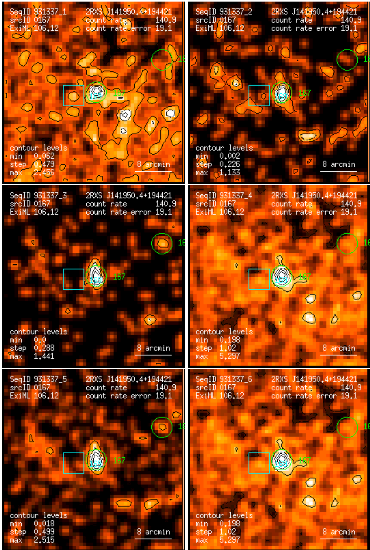
Figure 167: RASS 931337: detection 0167: band rate images, Gaussian filter: (1) PSPC channels 11 – 41, (2) 52 – 90, (3) 91 – 201, (4) 11 – 235, (5) 52 – 201, (6) 11 – 201. Broad band rates in counts/ks. Band rate contour levels in counts/ks/arcmin 2 .
