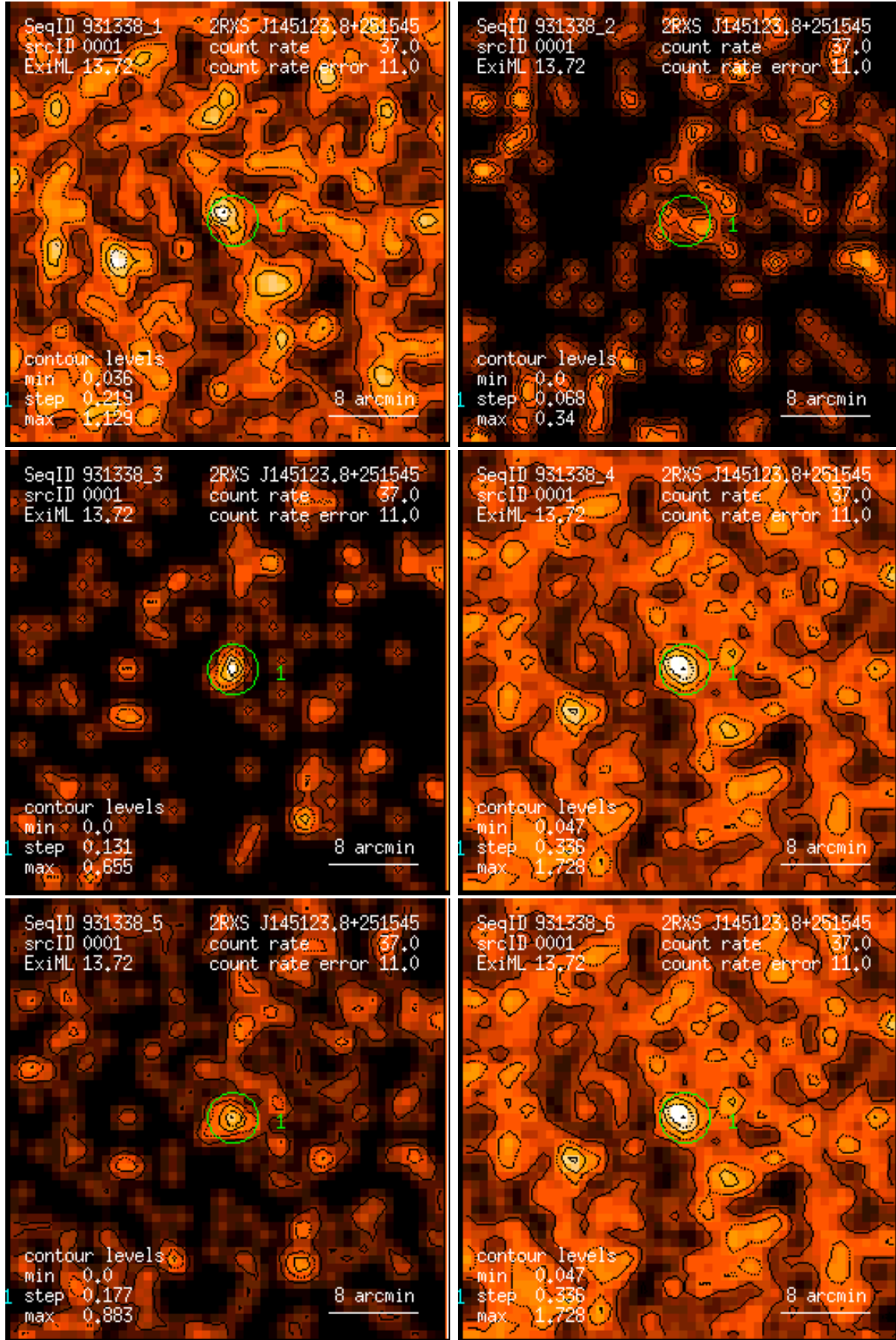
Figure 1: RASS 931338: detection 0001: band rate images, Gaussian filter: (1) PSPC channels 11 – 41, (2) 52 – 90, (3) 91 – 201, (4) 11 – 235, (5) 52 – 201, (6) 11 – 201. Broad band rates in counts/ks. Band rate contour levels in counts/ks/arcmin 2 .
